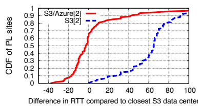
Figure 6: Comparison of second closest data center within a cloud service and across cloud services.
