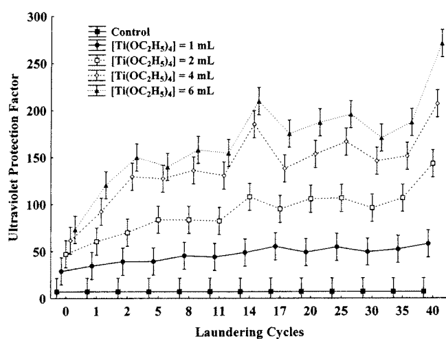
Figure 7 Fabric treated with titania nanosol: UPF versus laundering cycles.
