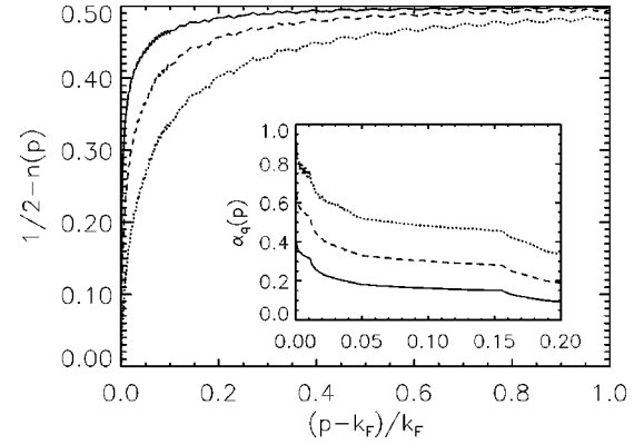
FIG. 1. Calculated momentum distribution function n(p) with respect to momentum p - k_F for a realistic QWR system of a = 70 nm. Solid, dashed, and dotted lines are results for three different interaction strengths V_0 = 1.21, 2.42, and 4.84 , respectively, where V_0 = 1.21 is for electron density 0.65 \times 10^6 \text{ cm}^{-1} and \epsilon_0 = 12.7 (Ref. 5). Inset: the effective exponent (around k_F ) obtained by taking the logarithmic derivative of the numerical n(p) for |p - k_F| < 0.2k_F .
