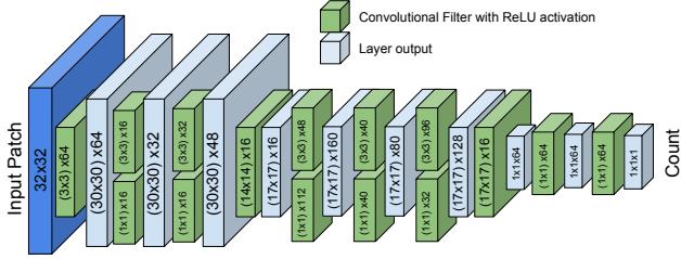
Figure 5: The Count-ception network architecture that is used for the regression network. Each intermediate tensor is labeled (filter size) x # filters. There are two points in the network where the size is reduced. The 3 \times 3 convolutions are padded so they do not reduce the size. Batch Normalization layers are inserted after each convolution but not pictured here.
