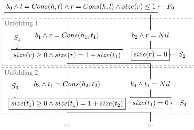
Figure 4. Decision tree for the verification condition of dup with two unfoldings and instrumented branching conditions.
