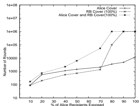
Fig. 2. Median rounds to identify a subset of Alice’s recipients. Background (BG) volume = 1700 messages/round. Mix delay probability P_{delay}=0.5
