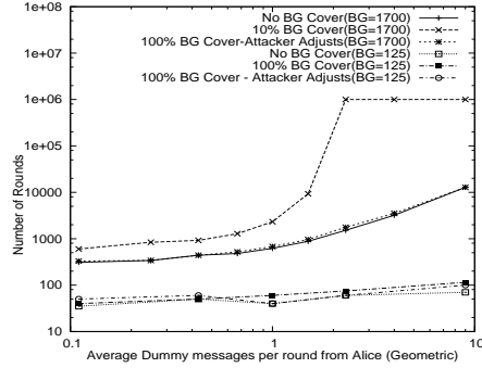
Fig. 3. Effect of Background Cover and Attacker Adjustment. Median rounds to guess 10 recipients.
