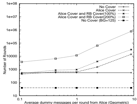
Fig. 6. Effect of RB cover traffic. Median rounds to guess 10 recipients. Background (BG) volume = 1700 messages/round.
