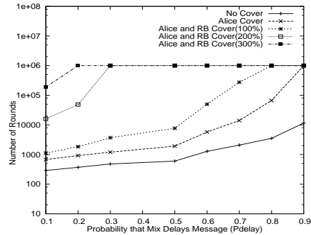
Fig. 8. Effect of increased delay distribution in the mix. Median rounds to guess 10 recipients. Background ( BG ) volume = 1700 messages/round.
