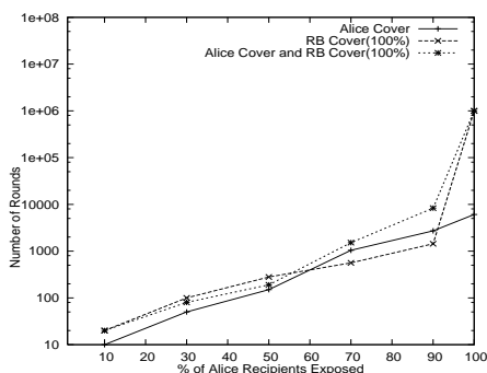
Fig. 1. Median rounds to identify a subset of Alice’s recipients. Background (BG) volume = 125 messages/round. Mix delay probability P_{delay}=0.5
