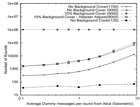
Fig. 4. Effect of increase in Background Volume. Median rounds to guess 10 recipients.
