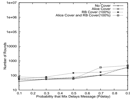
Fig. 7. Effect of increased delay distribution in the mix. Median rounds to guess 10 recipients. Background ( BG ) volume = 125 messages/round.
