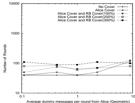
Fig. 5. Effect of RB cover traffic. Median rounds to guess 10 recipients. Background (BG) volume = 125 messages/round.
