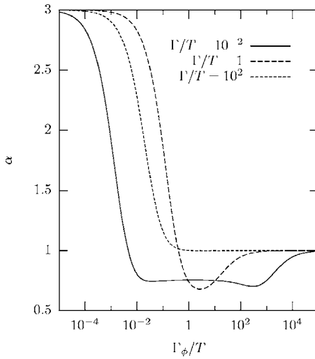
FIG. 2. Dependence of the Fano factor \alpha on the normalized decoherence rate \Gamma_\phi/T for three values of \Gamma/T .
