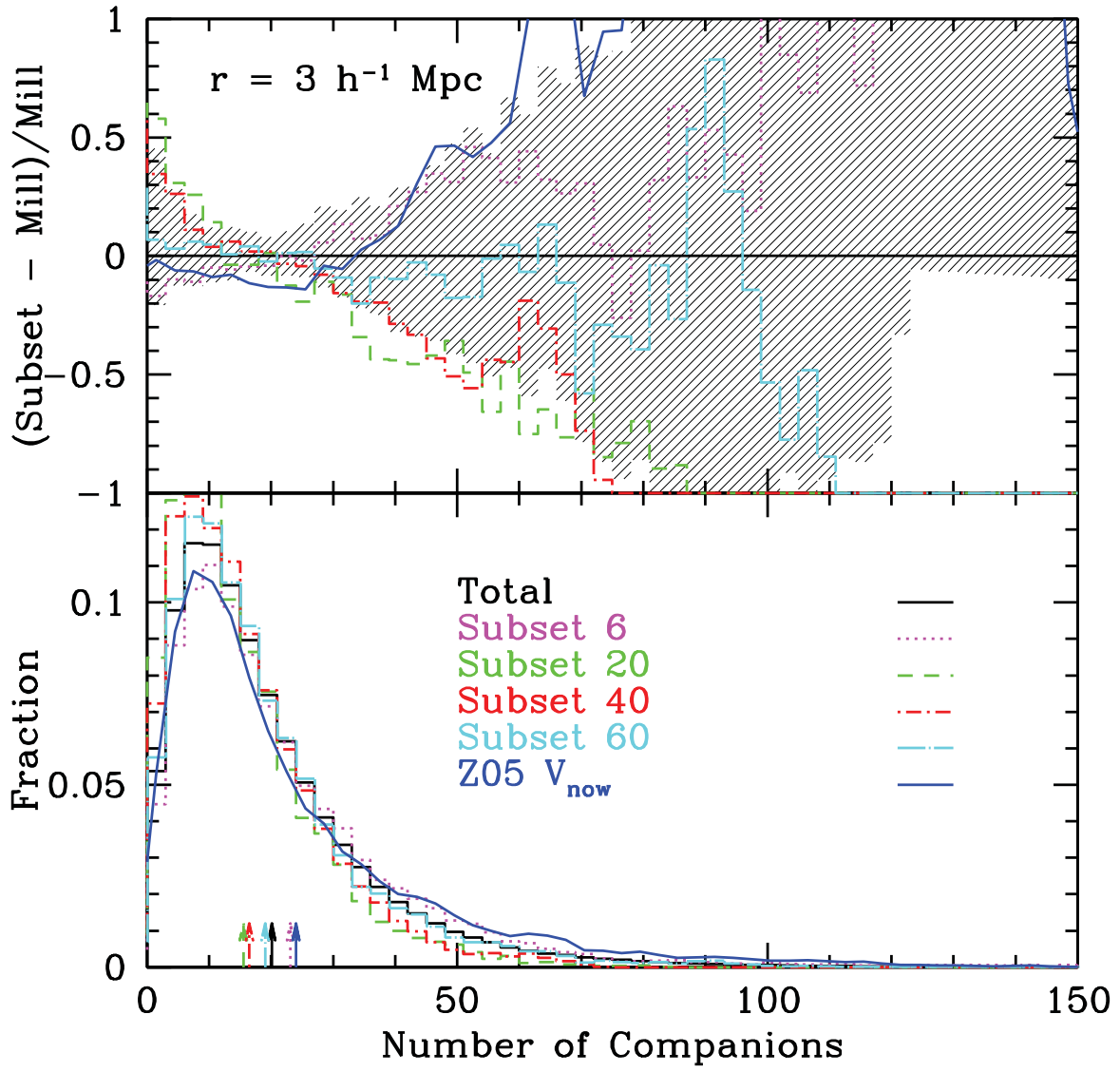
FIG. 3.— Comparison of counts-in-cylinders between the Millennium simulation and the Z05 model (smooth blue line) for the 3 \text{ h}^{-1} \text{ Mpc} cylinder. Bottom panel: Distribution of counts in R_c = 3 \text{ h}^{-1} \text{ Mpc} cylinders. The arrows denote the mean of each distribution. Top panel: Fractional deviation from the mean cylinder counts. The shaded area denotes the dispersion among the 64 sub-volumes of the Millennium simulation and provides a guideline for the statistical limitations of the comparison.
