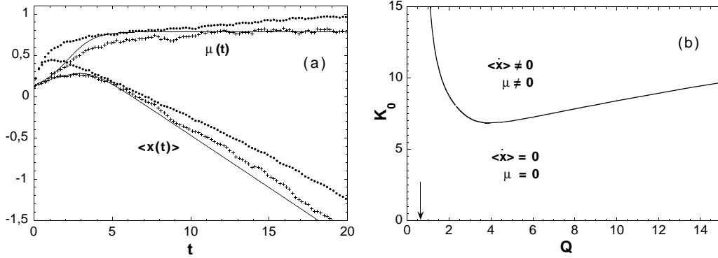
Fig. 1. – (a) Time evolution of \mu(t) from (13) and of \langle x(t) \rangle := \int x \rho(x, t) dx for the model (1)-(3) with T = 2, Q = 4, F = 0, K_0 = 10, A = 0.15 , and initial condition \rho(x, 0) = \delta(x - 0.1) . Solid line: N \rightarrow \infty by solving (4). Crosses: N = 1024 by simulating (1), averaged over 10 realizations. Dots: simulations with nearest neighbor instead of global coupling in (1) for a 64 \times 64 square lattice with periodic boundary conditions, averaged over 10 realizations, and modified parameters Q = 10, K_0 = 20 . (b) Phase diagram for (1)-(3) with T = 2, F = 0, A = 0.15 , and N \rightarrow \infty . \langle \dot{x} \rangle is the particle current and \mu the order parameter (13) in the steady state t \rightarrow \infty . Arrow: asymptotic phase boundary (12) for K_0 \rightarrow \infty .
