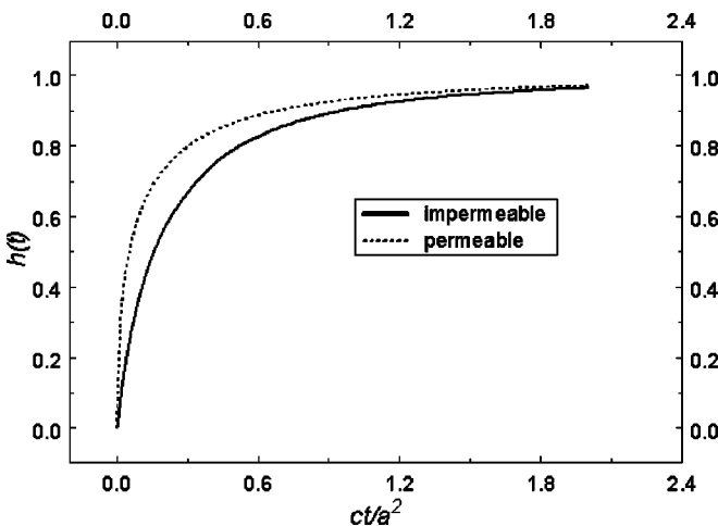
Fig. 21 Time dependence of the boundary shear strain for uniform shear stress applied to a spherical cavity
