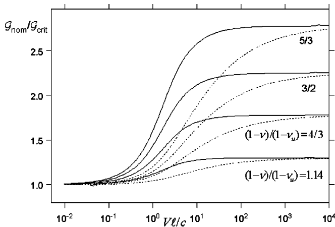
Fig. 16 Curves of \mathcal{G}_{nom}/\mathcal{G}_{crit} against Vl/c for four values of the ratio (1-\nu)/(1-\nu_u) . For large values of Vl/c , \mathcal{G}_{nom}/\mathcal{G}_{crit} approaches the square of this ratio. Dashed curves are for permeable and solid for impermeable.
