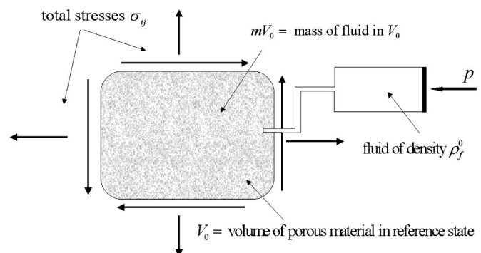
Fig. 1 Schematic illustration of an element of porous material connected to an imagined reservoir of homogeneous pore fluid
