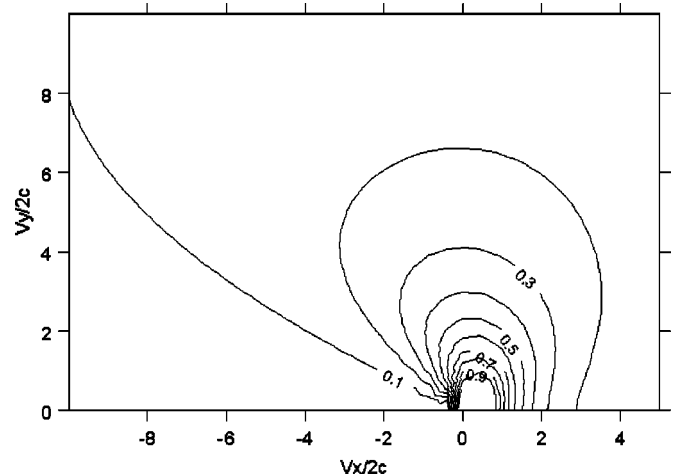
Fig. 9 Contours of nondimensional pore pressure for a shear dislocation moving steadily on an impermeable plane
