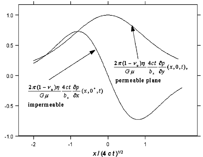
Fig. 5 Pore pressure gradient (proportional to negative of fluid mass flux) on y=0 in the y direction for a shear dislocation on a permeable plane and in x direction for a shear dislocation on an impermeable plane
