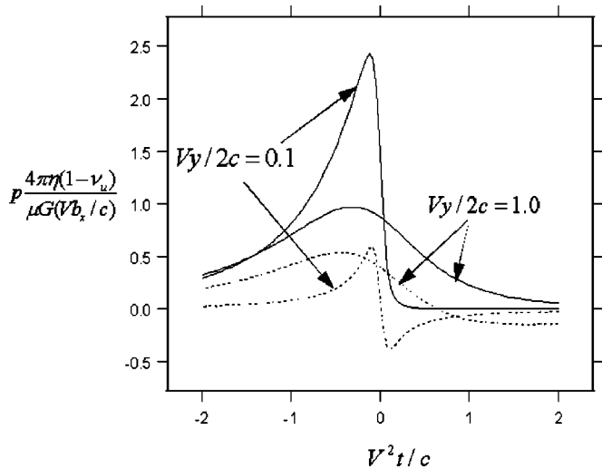
Fig. 7 Pore pressure (in nondimensional form) vs the nondimensional time V^2t/c for dislocations moving steadily on permeable (dashed) and impermeable (solid) planes
