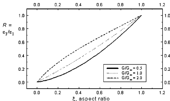
Fig. 18 Variation of strain state with aspect ratio and mismatch of shear modulus for pressure changes
