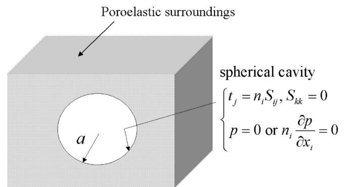
Fig. 20 Sketch of a spherical cavity in an infinite poroelastic solid. Cavity boundary is loaded by a traction derived from a uniform deviatoric stress, S_{ij} , S_{kk} = 0 . Cavity boundary is either permeable ( p = 0 ) or impermeable ( \partial p/\partial n = 0 ).
