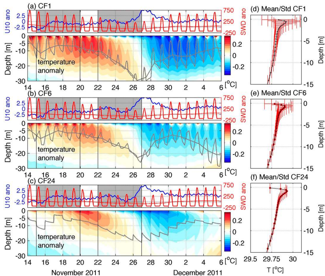
FIG. 6. (left) Time–depth diagrams of the upper-ocean temperature anomalies (shading, °C) averaged over the NSA region (0.7°S–7°N, 73°–80.5°E) from (a) CF1, (b) CF6, and (c) CF24, overlaid with the respective depth of turbulent boundary layer (TBL; m, gray contours). Both the hourly- and daily-mean TBL values are shown in (a) and (b). Blue and red lines denote the anomalous 10-m zonal wind ( \text{m s}^{-1} ) and the downward shortwave radiation at the surface ( \text{W m}^{-2} ), respectively. The anomalies are with respect to the 30-day mean. (right) The mean upper-ocean temperature profiles for (d) CF1, (e) CF6, and (f) CF24 are overlaid with \pm 1 intradiurnal standard deviation (STD) for the suppressed phase of MJO2 (14–21 Nov 2011).
