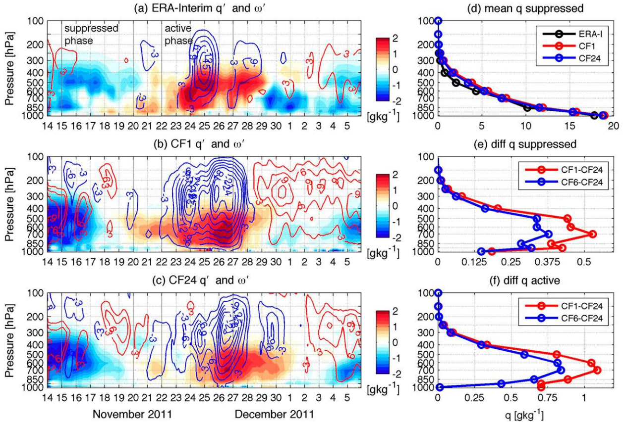
FIG. 9. Pressure–time cross sections of the anomalous specific humidity ( q' ; \text{g kg}^{-1} ) over the NSA region (0.7°S–7°N, 73°–80.5°E) from (a) ERA-Interim, (b) CF1, and (c) CF24. The anomalies are respect to the 30-day-mean values. Contours denote the pressure velocity anomaly ( \omega' ; \text{CI} = 10 \text{ hPa h}^{-1} ) with the blue (red) representing the ascending (descending) motion. (d) The time-mean specific humidity profiles during the suppressed phase of MJO2. Also the differences in the mean specific humidity are shown for the (e) suppressed and (f) active phases.
