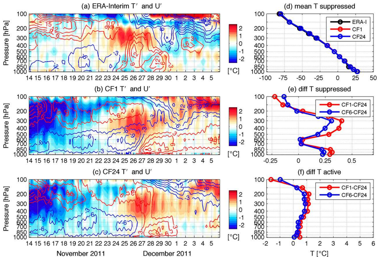
FIG. 10. As in Fig. 9, but for temperature anomaly ( T' , colors; °C) and zonal wind anomaly ( U' , contours; \text{CI} = 3 \text{ m s}^{-1} ). The red (blue) contours denote westerly (easterly) wind anomalies.
