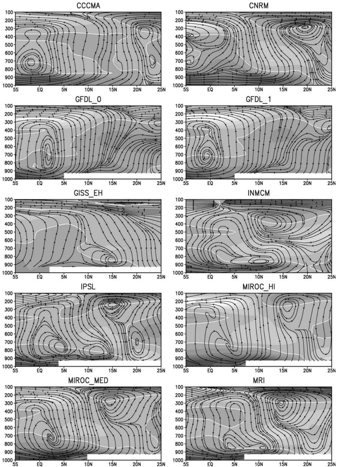
FIG. 6. JJAS streamline cross sections ( v ; w_g \cdot 10^{-2} ) at 5^\circ\text{E} in some coupled GCM integrations.
