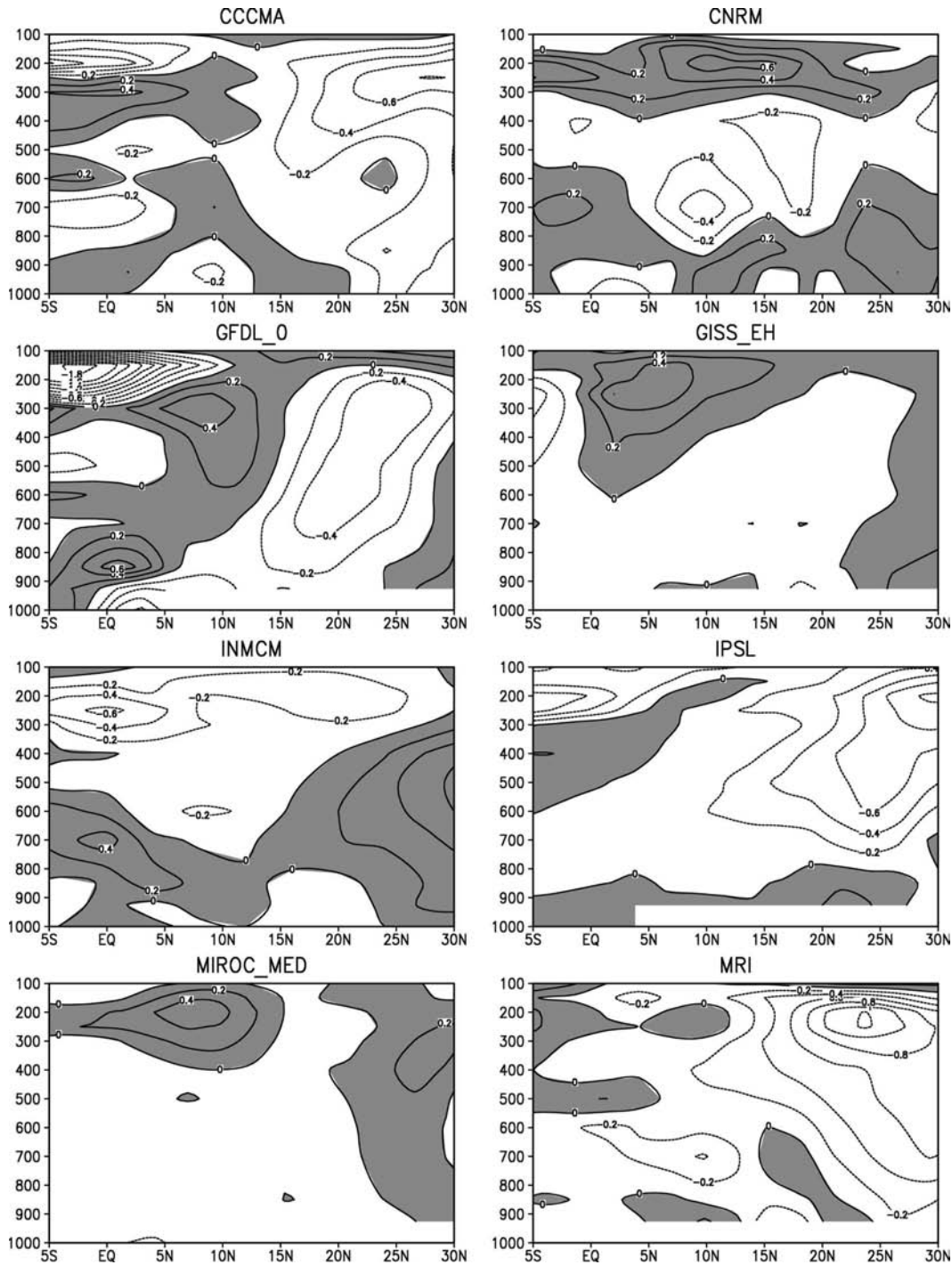
FIG. 10. Same as in Fig. 8, but for summer meridional velocity at 5^{\circ}\text{E} from coupled GCM integrations. Contours are every 0.2 \text{ m s}^{-1} , and shading denotes negative values.
