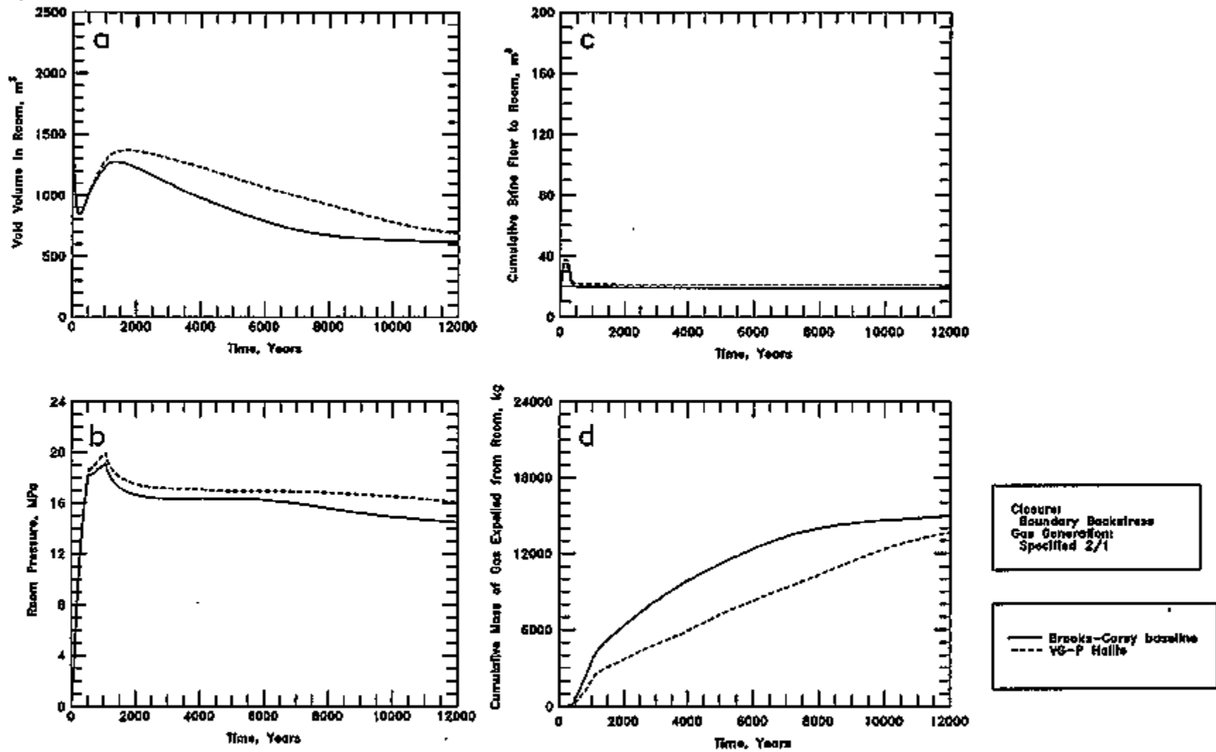
Figure 5-14 (a-d). Sensitivity to halite two-phase characteristic relationship: a - Void Volume; b - Gas Pressure; c - Brine Flow; d - Gas Expulsion.
