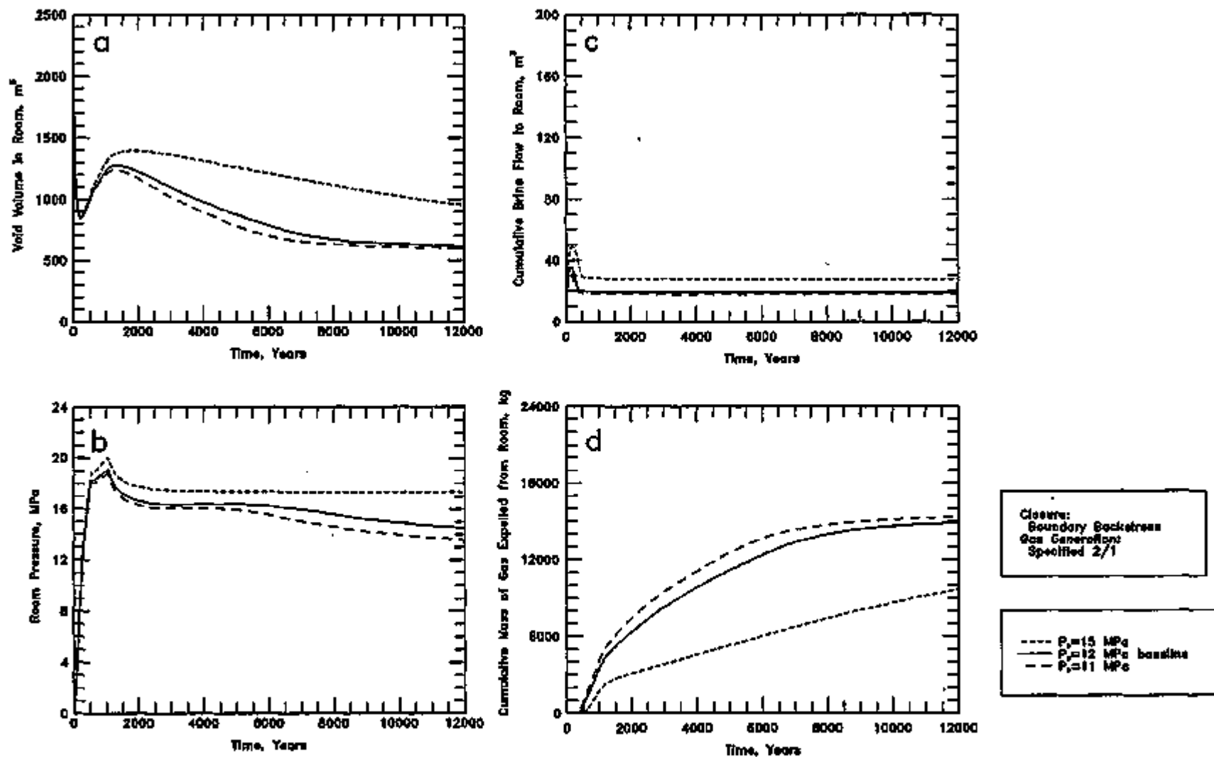
Figure 5-12 (a-d). Sensitivity to initial Salado Formation pressure: a - Void Volume; b - Gas Pressure; c - Brine Flow; d - Gas Expulsion.
