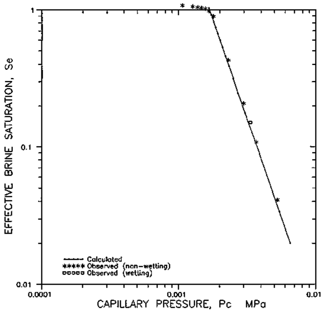
Figure 3. Observed and calculated effective saturation vs. capillary pressure used to determine the Brooks and Corey (1964) model parameters, \lambda (slope) and P_c (intercept at S_e = 1 ).
