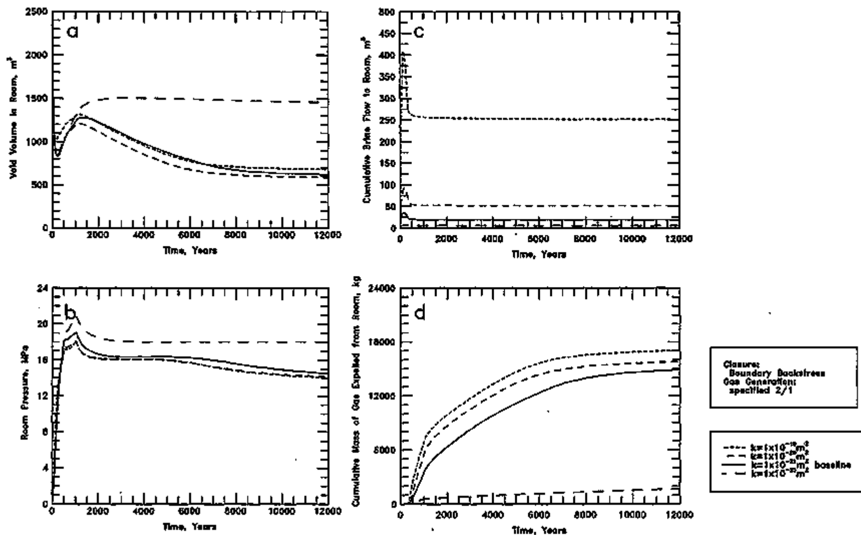
Figure 5-10 (a-d). Sensitivity to halite intrinsic permeability (constant threshold pressure): a - Void Volume; b - Gas Pressure; c - Brine Flow; d - Gas Expulsion.
