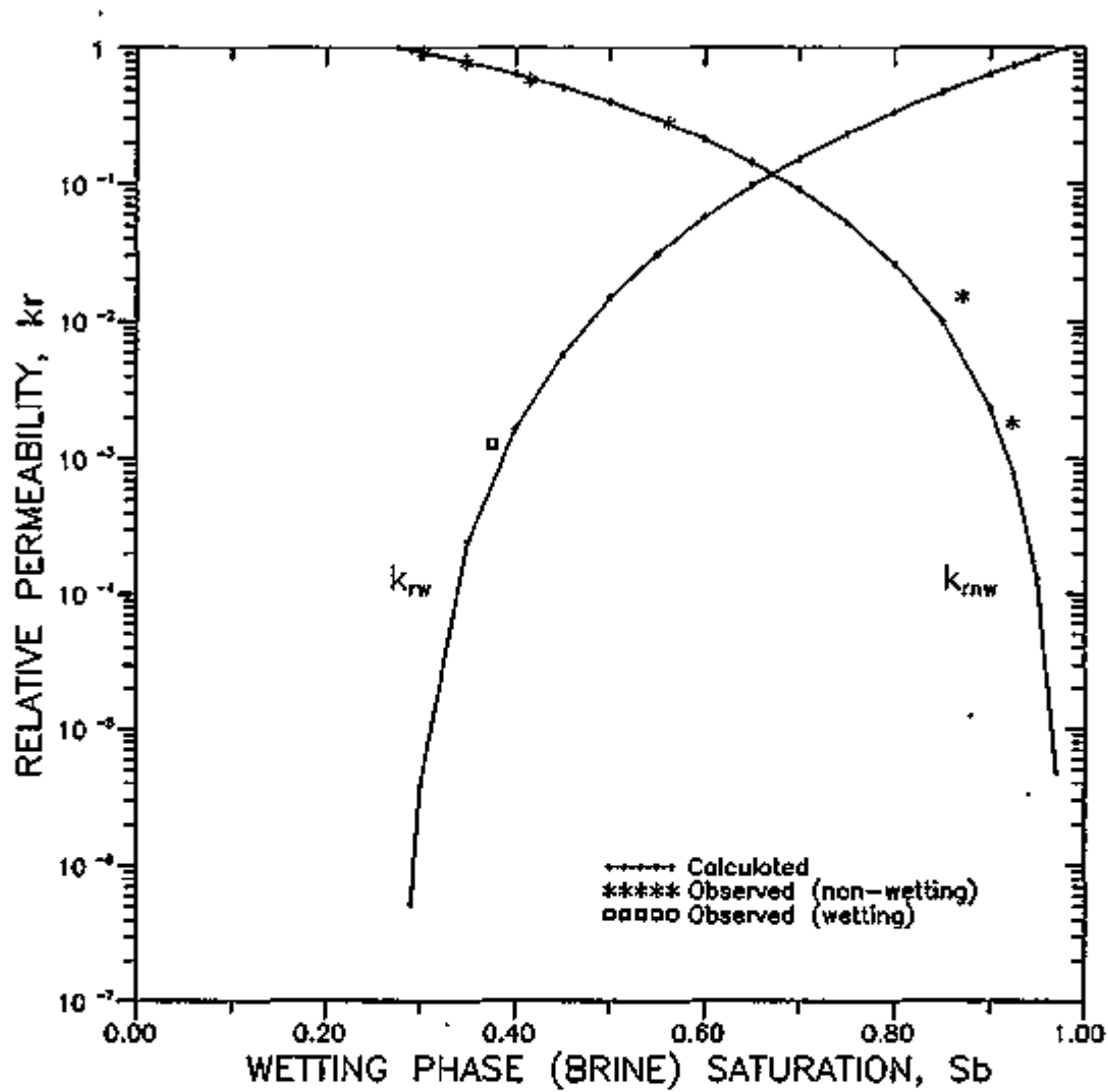
Figure 2. Observed relative permeabilities for the fragmented mixture and calculated relative permeabilities for the waste disposal room (log scale).
