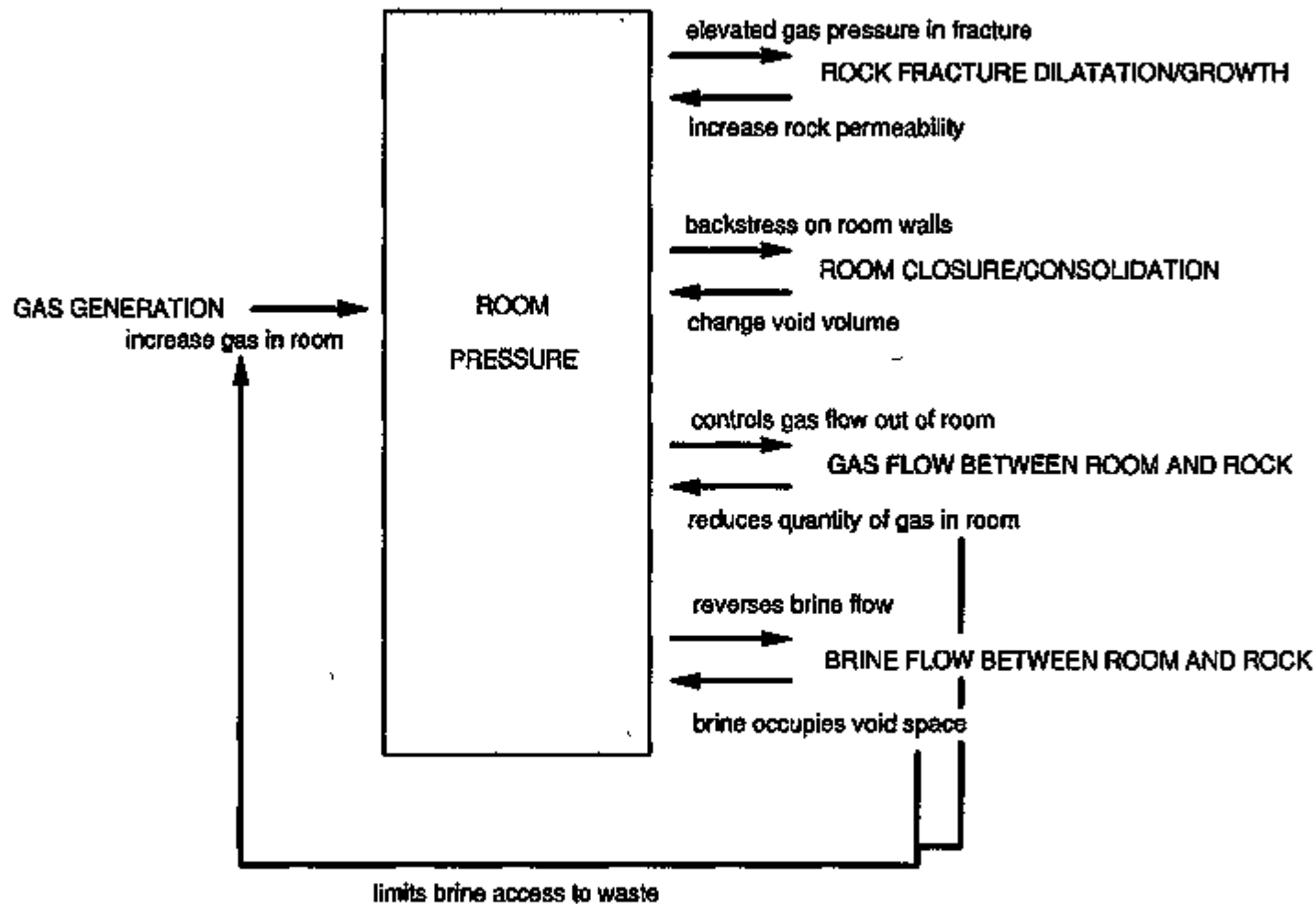
Figure 1-9. Schematic illustration of the chemical, hydrologic, and mechanical coupling that control repository response to waste-generated gas (after Davies et al., 1992).
