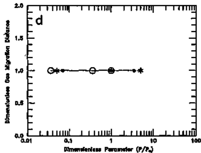
Figure 5-3 (a-d). Dimensionless plots of performance measure sensitivity to disposal room multiphase flow properties: a - Maximum Room Pressure; b - Maximum Brine in Room; c - Gas Expulsion; d - Gas Migration Distance.
