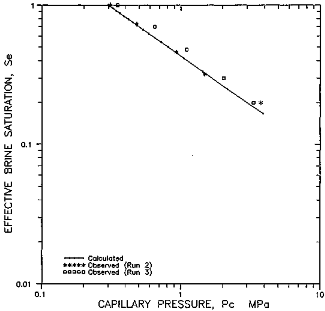
Figure 4. Observed and calculated effective saturation vs. capillary pressure used to determine the Brooks and Corey (1964) model parameters, \lambda (slope) and P_c (intercept at S_e = 1 ).
