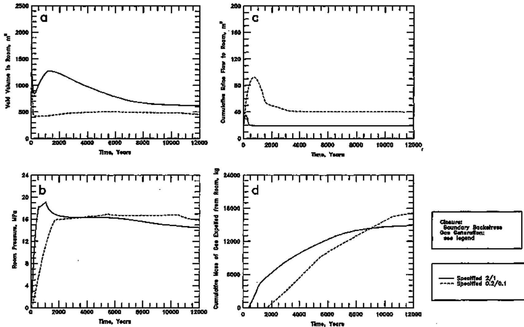
Figure 4-1 (a-d). TOUGH2/EOSS boundary backstress simulation results for coupled flow and closure under best estimate conditions: a - Void Volume; b - Gas Pressure; c - Brine Flow; d - Gas Expulsion.
