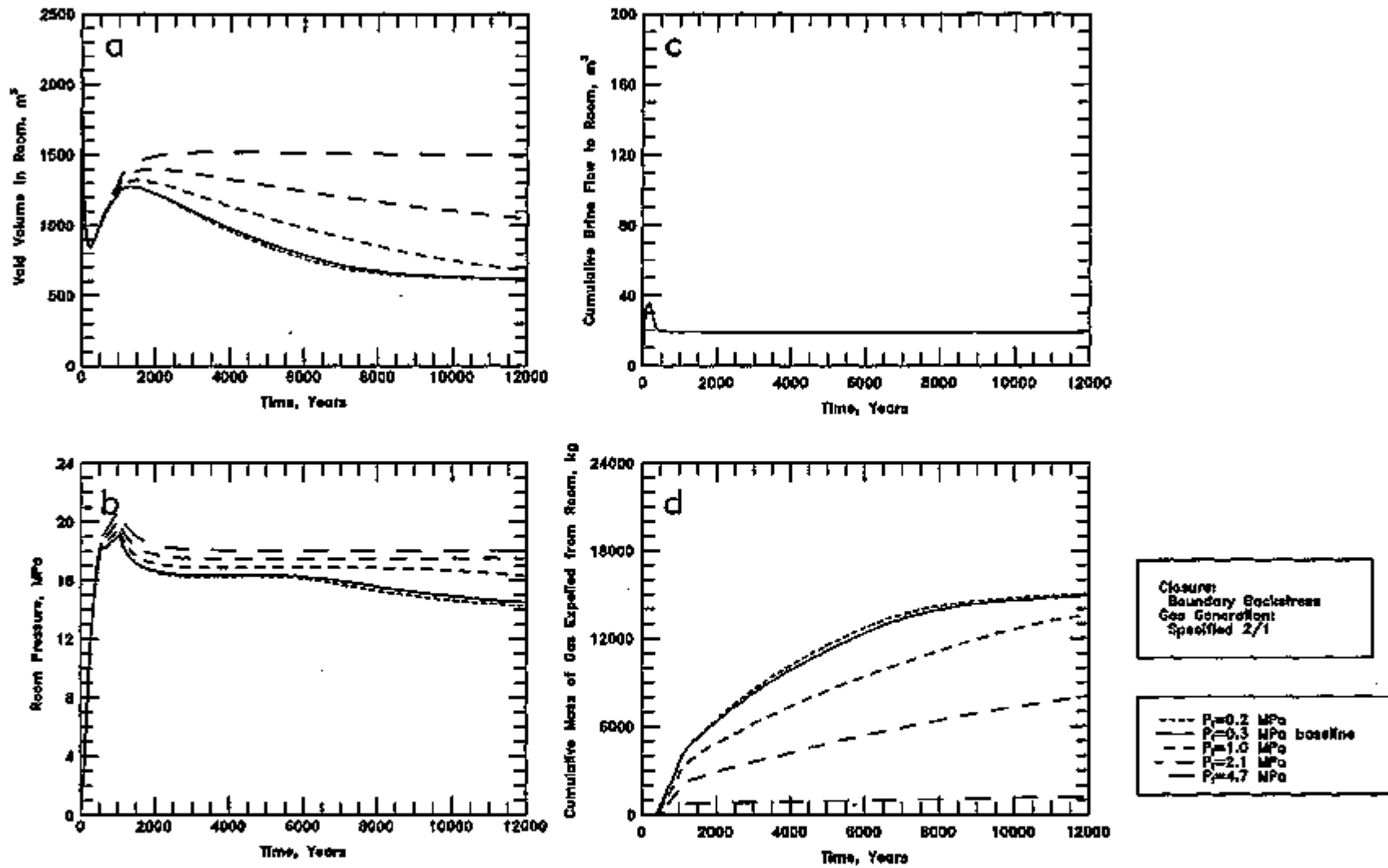
Figure 5-22 (a-d). Sensitivity to interbed threshold pressure: a - Void Volume; b - Gas Pressure; c - Brine Flow; d - Gas Expulsion.
