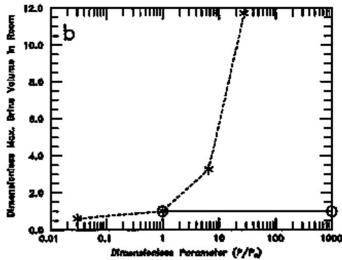
Figure 5-2 (a-d). Dimensionless plots of performance measure sensitivity to disposal room intrinsic permeability and initial brine saturation: a - Maximum Room Pressure; b - Maximum Brine in Room; c - Gas Expulsion; d - Gas Migration Distance.
