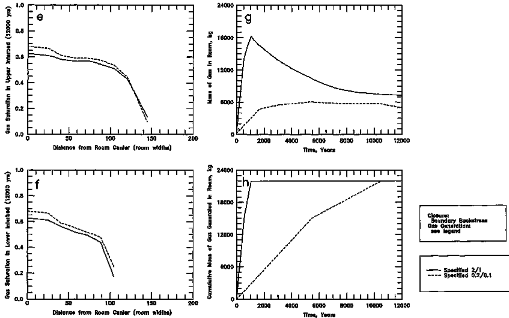
Figure 4-1 (e-h). TOUGH2/EOS8 boundary backstress simulation results for coupled flow and closure under best estimate conditions: e - Upper Interbed Gas Profile; f - Lower Interbed Gas Profile; g - Room Gas Mass; h - Gas Generation.
