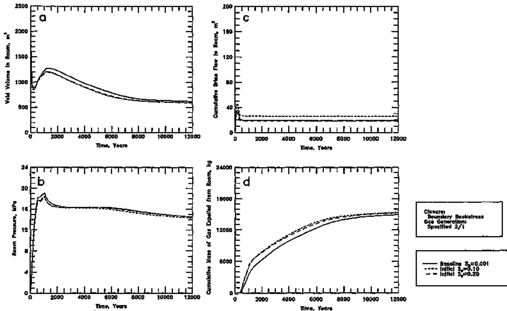
Figure 5-33 (a-d). Results from gas exsolution alternative conceptual model: a - Void Volume; b - Gas Pressure; c - Brine Flow; d - Gas Expulsion.
