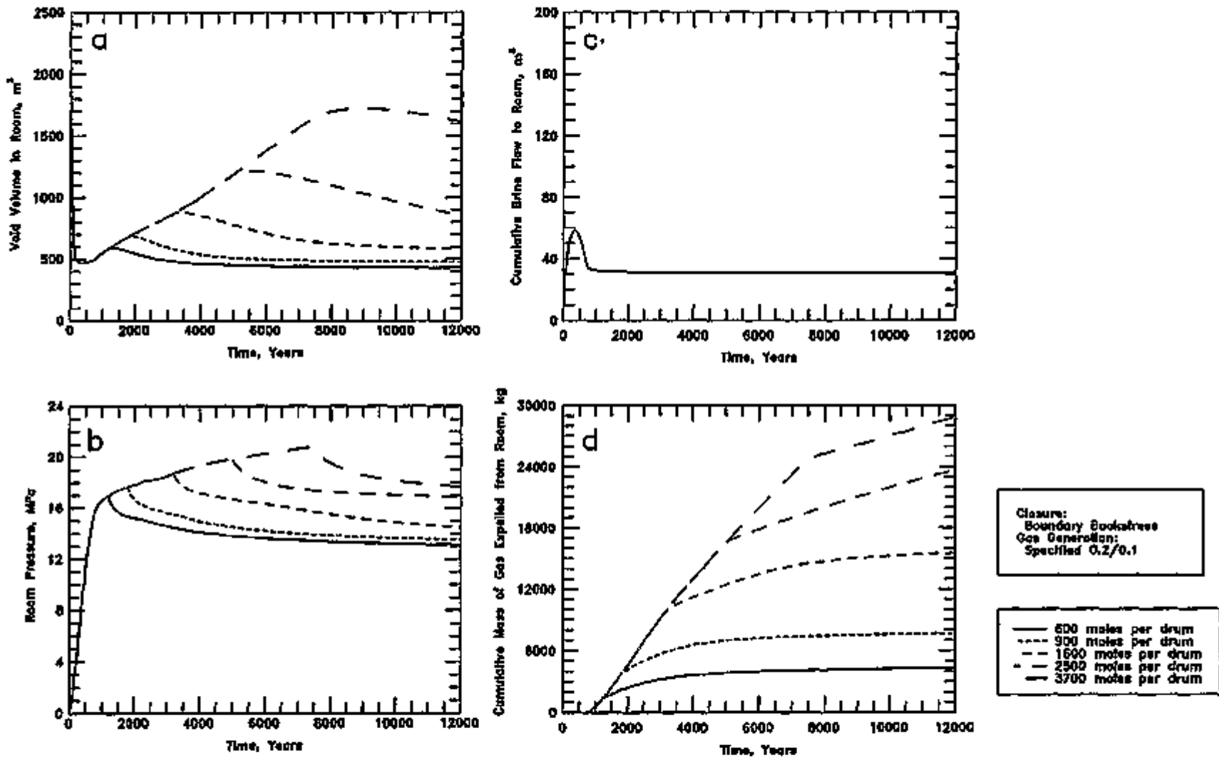
Figure 5-27 (a-d). Sensitivity to gas-generation potential: a - Void Volume; b - Gas Pressure; c - Brine Flow; d - Gas Expulsion.
