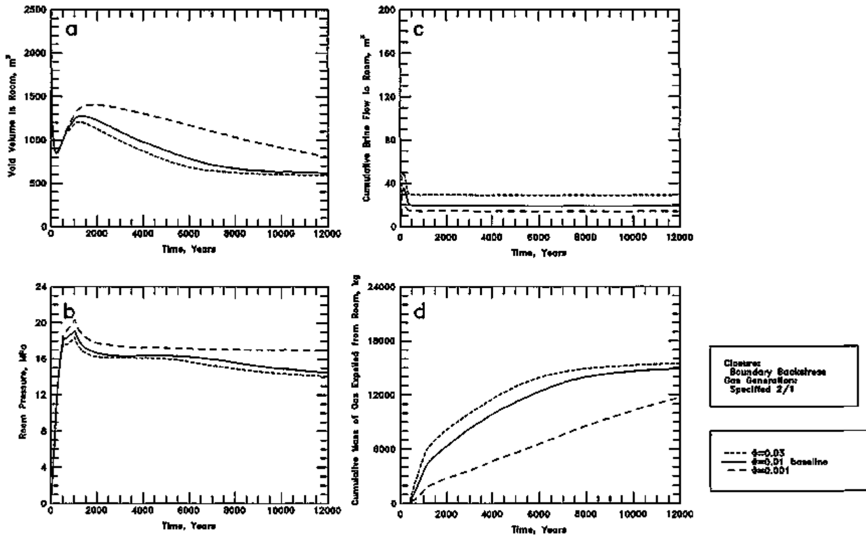
Figure 5-11 (a-d). Sensitivity to halite porosity (constant pore volume compressibility): a - Void Volume; b - Gas Pressure; c - Brine Flow; d - Gas Expulsion.
