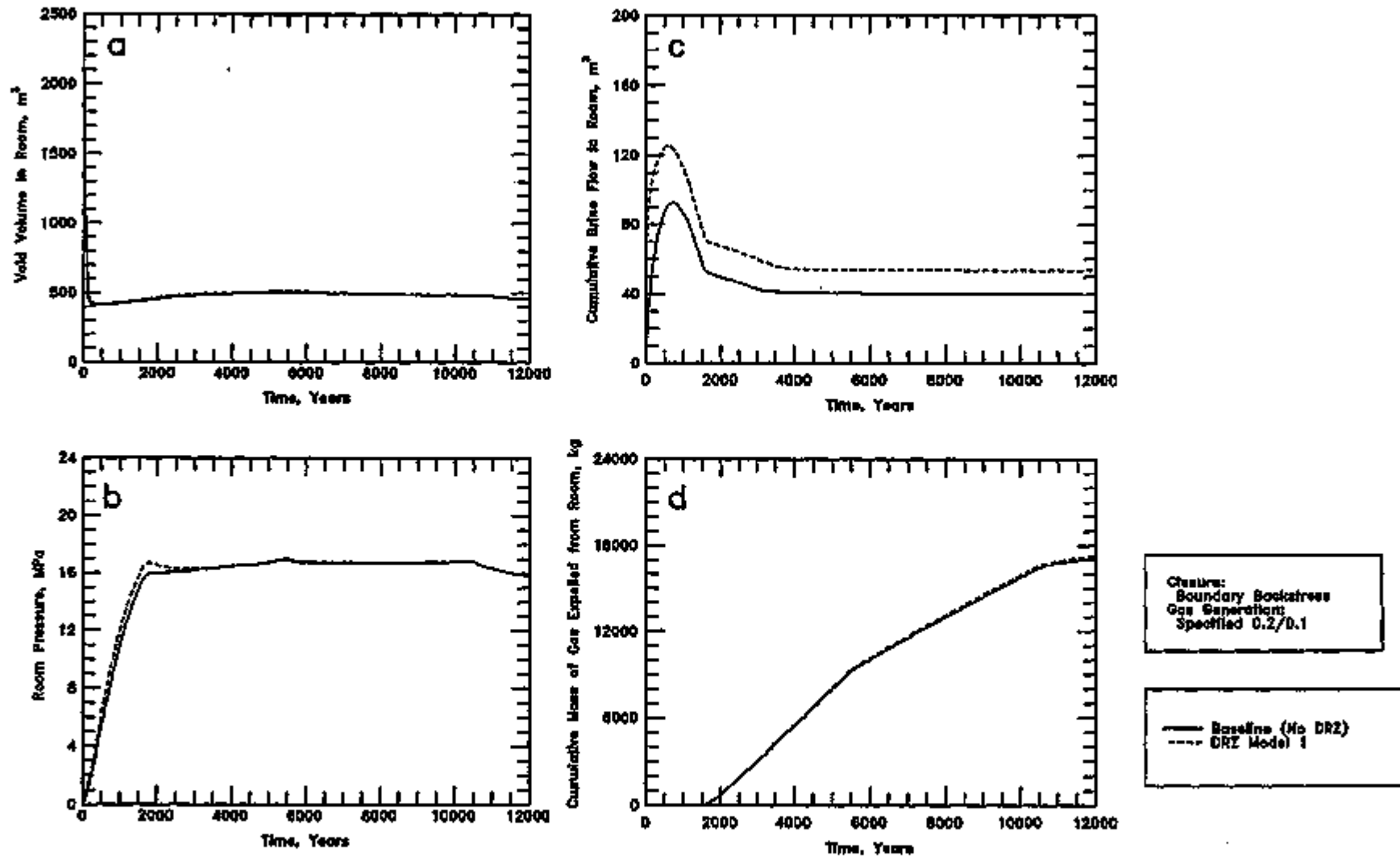
Figure 5-31 (a-d). Results from Disturbed Rock Zone alternative conceptual model: a - Void Volume; b - Gas Pressure; c - Brine Flow; d - Gas Expulsion.
