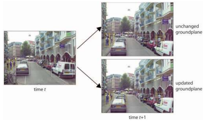
Fig. 2. Illustration of the importance of a continuous reestimation of scene geometry. The images show the effect on object detection when the vehicle hits a speed bump (top) if using an unchanged ground plane estimate and (bottom) if using the online reestimate.
