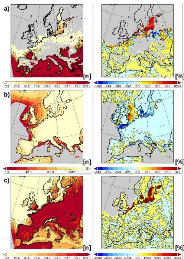
580 Figure 5: a) left: Number of tropical nights diagnosed from the coupled regional ocean atmosphere model during the reference period 1970-1999. right: Difference [%] of the coupled minus the uncoupled model. b) same as a) but for the number of frost days. c) left: number of periods of at least 3 consecutive warm days (days where the daily maximum temperature exceeds 20°C). right: Difference [%] of the coupled minus the uncoupled model.
