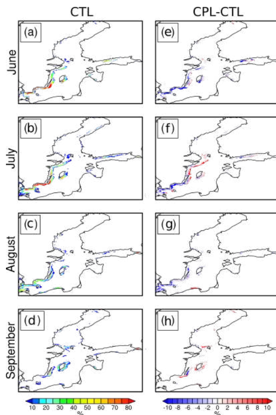
950 Fig. 7: The left column shows the upwelling frequency during June to September, 2015, the right column shows the difference between the simulation considering wave influence and the control experiment (Figure is adapted from Wu et al., 2019b).
