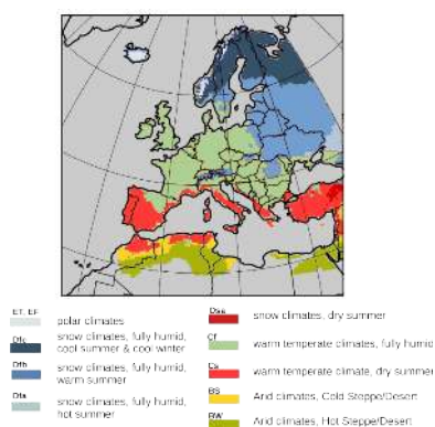
110 Figure 1: Climate classification based on E-OBS monthly mean temperature and precipitation (Cornes et al., 2018). Classes are defined after Köppen (1923).
