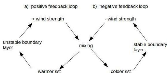
485 Figure 4:a) positive winter feedback loop. b) negative summer short circuit. Drawn after Gröger et al. (2015).
