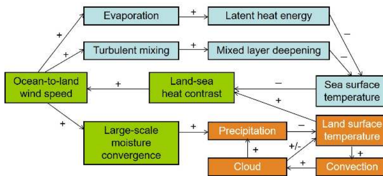
635 Figure 6: Air-sea feedback and interaction diagram. For each arrow, the initial status indicates that the source quantity is increasing, and the sign (– or +) indicates the changing tendency of the target quantity. Colours denote the group of changes or states over sea (blue), land (brown) and the land-sea interactions (green). [Source: Ho-Hagemann et al. (2017)]
