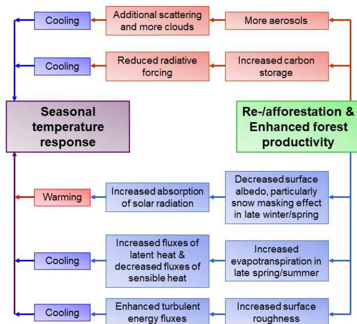
300 Fig. 2: Outline of the biogeochemical (upper part in brown) and the biophysical influence (lower part in blue) of re-/afforestation or enhanced forest productivity in the Baltic Sea region on near-surface temperatures. The overall effect on near-surface temperatures varies by season and region, depending, for instance, on snow cover and incoming solar radiation (adapted from May et al. (2020)).
