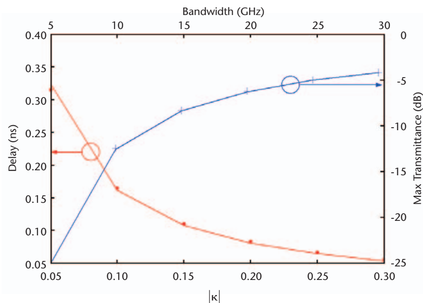
Figure 3. Tradeoffs among delay (red), losses (blue) and bandwidth for a CROW consisting of 10 coupled ring resonators having a FSR of 310 GHz and propagation loss of 4 dB/cm.
