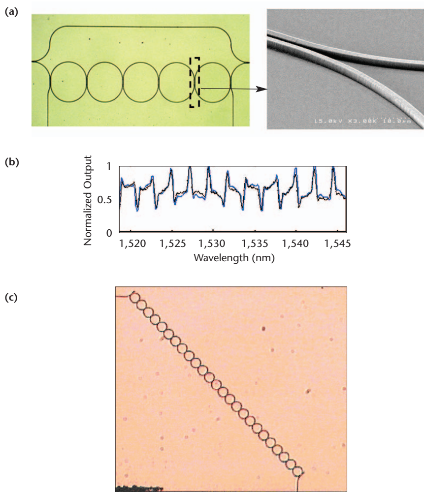
Figure 4. (a) Optical image of the CROW-MZI and SEM zoom of the coupling region; (b) Theoretical fit ( blue ) and a measurement ( black ) of the CROW-MZI transmission. The fit parameters are \kappa = 0.46 and loss is 30 dB/cm; (c) CROW consisting of 25 resonators.
