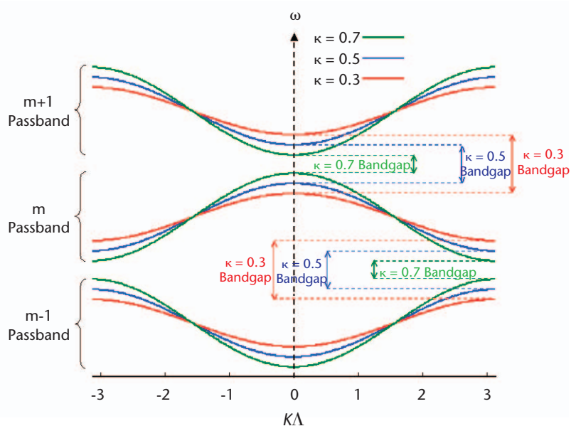
Figure 2. Dispersion curves for an infinite CROW for intracavity coupling ratios of 0.3 (red), 0.5 (blue) and 0.7 (green).
