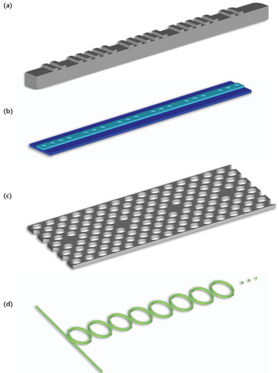
Figure 1. Various implementations of CROWs: (a) coupled Fabry-Pérot cavities; (b) one-dimensional (1D) coupled photonic crystal defects; (c) 2D coupled photonic crystal defects; (d) coupled microring resonators.
