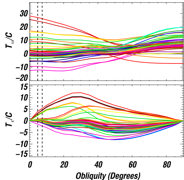
Figure 6. The obliquity (bottom) and the spin (top) torques (YORP curves) through which the aggregate object in simulation 14 (Figure 5) evolves. The torque components divided by the moment of inertia (in units of 10^{-18} \text{ s}^{-2} ) are plotted against the obliquity in degrees. Each colored curve corresponds to a new shape of the aggregate object after a movement of material, and corresponds to the segment of the same color in Figure 5. Dashed vertical lines indicate the range of obliquity values to which the object is confined during the evolution. The spin and the obliquity torques are symmetric and antisymmetric about 90^\circ , respectively.
