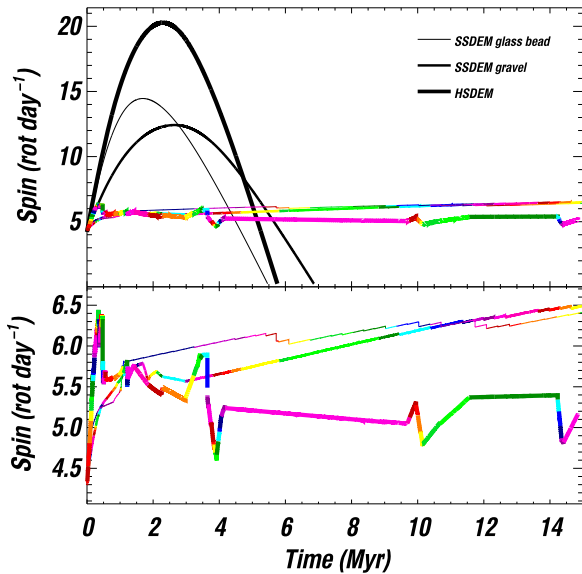
Figure 18. Spin evolutions obtained for simulation 10 using HSDEM and SSDEM with the coefficients of static and rolling frictions of gravel and glass beads. Black lines show the rigid-body evolution (top). Colored lines show the evolution of the aggregate (top and bottom). Small variations of the aggregate evolution can be noticed in the bottom panels. Note that self-limitation of the YORP effect still occurs in the SSDEM simulations. As in the HSDEM case, the SSDEM-simulated objects evolve through a sequence of shape changes that limit the spin and prevent the YORP cycle from completing.
