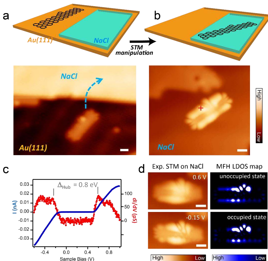
Fig. 2 Electronic properties of the edge-extended 7AGNR on NaCl/Au(111). Schemes and STM images a , before and b , after transferring an edge-extended 7AGNR segment from the Au(111) surface onto a NaCl insulating layer by STM manipulation ( a : V_s = -0.1 V, I_t = 10 pA; b : V_s = -0.5 V, I_t = 5 pA). Scale bar: 1 nm. c , Differential conductance ( dI/dV -V) and simultaneously acquired current ( I -V) spectra recorded above the edge extension (indicated by a red cross in b ), revealing a Hubbard gap of \sim 0.8 eV. d , STM images acquired at 0.6 V and -0.15 V, and the corresponding MFH simulated LDOS maps. Scale bar: 1 nm.
