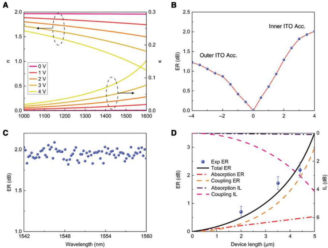
Figure 3: Simulated and experimental results for the ITO coupling-enhanced modulator.
