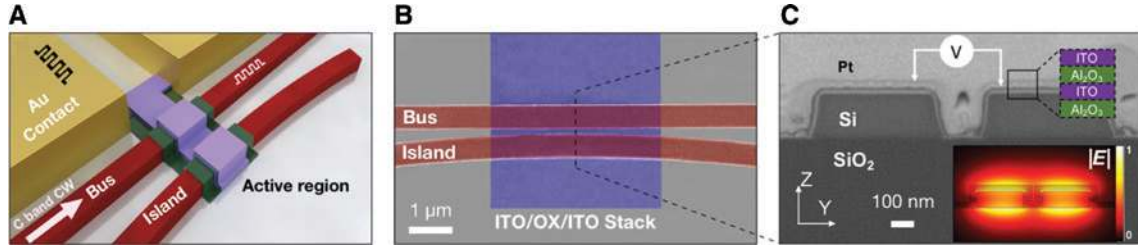
Figure 2: Device configuration of the coupling-enhanced modulator.
