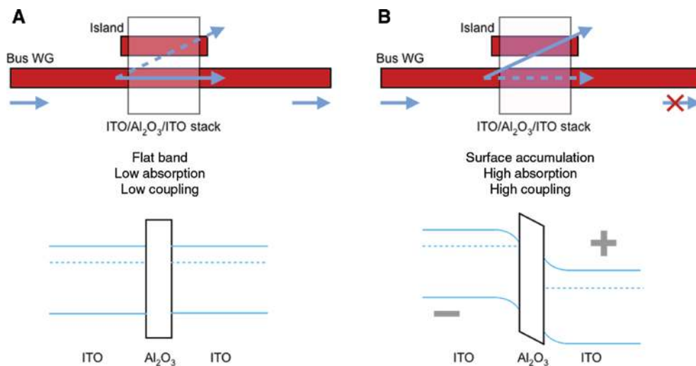
Figure 1: Operation principle for a coupling-enhanced ITO modulator; here the changes of both ITO absorption and coupling coefficient contribute synergistically to the modulation of the transmission on the bus waveguide, thus exploiting the Kramers-Kronig relations to achieve higher modulation performance as experimentally demonstrated in this work.
