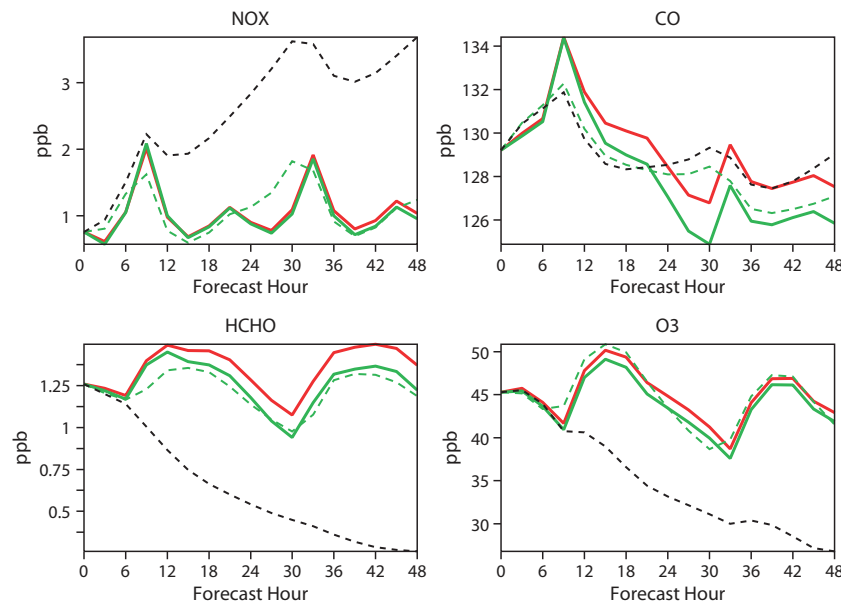
Fig. 2. Time series (forecast hour) of the area-averaged \text{NO}_x , CO, HCHO and \text{O}_3 -concentrations over Europe at about 240 m simulated with the MOZART-3 (red), and simulated with the IFS applying MOZART-3 tendencies in total-tendency mode (green, solid), in surface-flux mode (green-dashed) and no application of tendencies (black, dotted). The coupled IFS tracer simulation (green) imitates that of the CTM MOZART-3 (green) in a satisfactory way.
