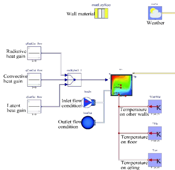
Figure 6 Diagram of Modelica models for the mixed convection.
