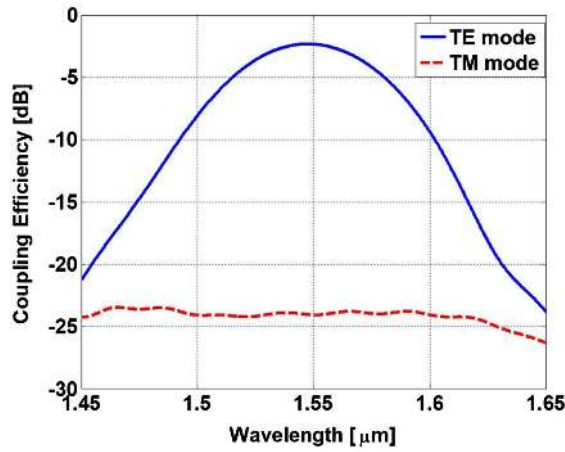
Fig. 19. CE of a TE-optimized 1D-GC as a function of optical wavelength for TE light polarization (blue trace) and for TM light polarization (red trace).
