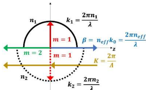
Fig. 15. Wave-vector diagrams of waveguide GCs in resonant configuration.
