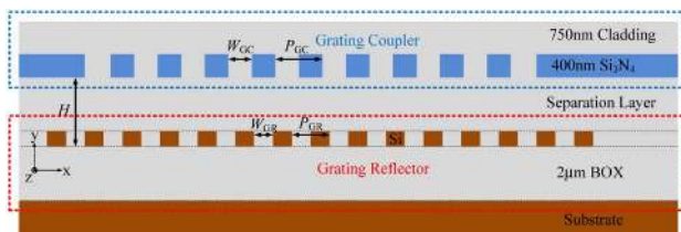
Fig. 41. Cross-sectional schematic of the \text{Si}_3\text{N}_4 -on-SOI dual-level GC reported in [98]. Reproduced from [98].
