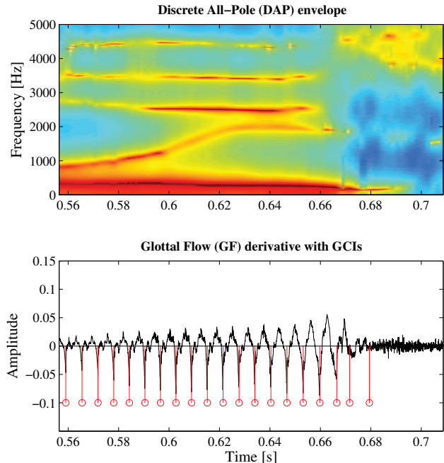
Fig. 2. Example showing analysis of a short speech segment using basic functionalities of COVAREP: DAP spectral envelope representation (top panel) and glottal flow derivative estimation along with glottal closure instants (bottom panel).
