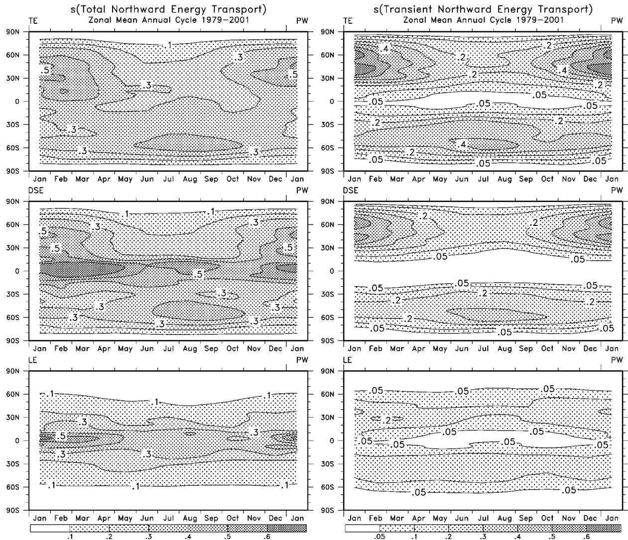
FIG. 10. Standard deviations of total zonal mean northward energy transport for 1979–2001 for the mean annual cycle from Fig. 3, for (top) TE, (middle) DSE, and (bottom) LE, for the total (left) and transients (right), with shadings given in the key. The contour interval is 0.1 PW with 0.05 PW in some panels.
