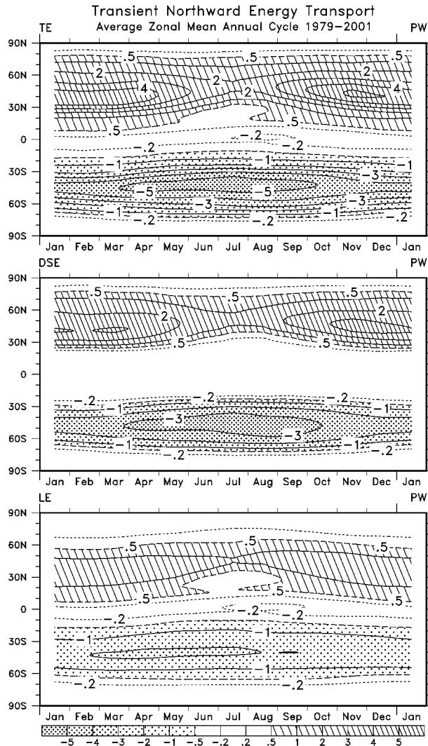
FIG. 4. Zonal mean northward energy transport by the transient eddies for 1979–2001 for the mean annual cycle, in PW. Shown are the atmospheric energy transports for the (top) TE, (middle) DSE, and (bottom) LE, with shadings given in the key. The contour interval varies but the same key applies to each panel.
