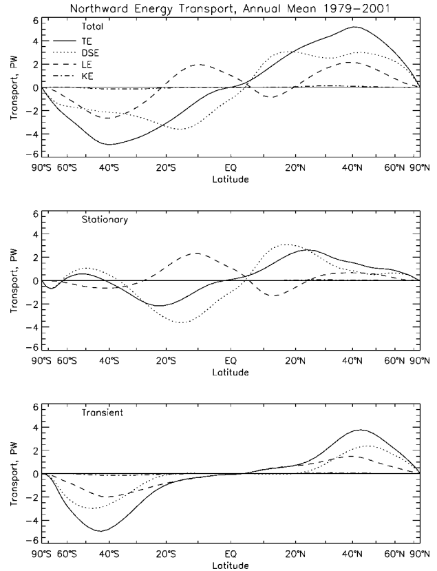
FIG. 1. Annual and zonal mean for 1979–2001 northward energy transport for the (top) total atmospheric energy, (middle) quasi-stationary component, and (bottom) transient component, showing the total, dry static, and kinetic energy components; in PW. The coordinate is latitude ( \phi ) plotted as \sin\phi so that values properly depict the area.
