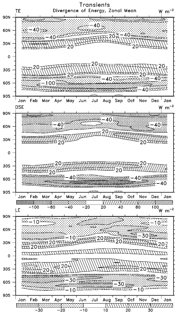
FIG. 6. Divergence of zonal mean northward energy transport by the transient eddies for 1979–2001 for the mean annual cycle, in W m^{-2} . Shown are the (top) TE, (middle) DSE, and (bottom) LE, with shadings given in the keys. The contour interval is 20 W m^{-2} in the top two panels and 10 W m^{-2} in the bottom panel.
