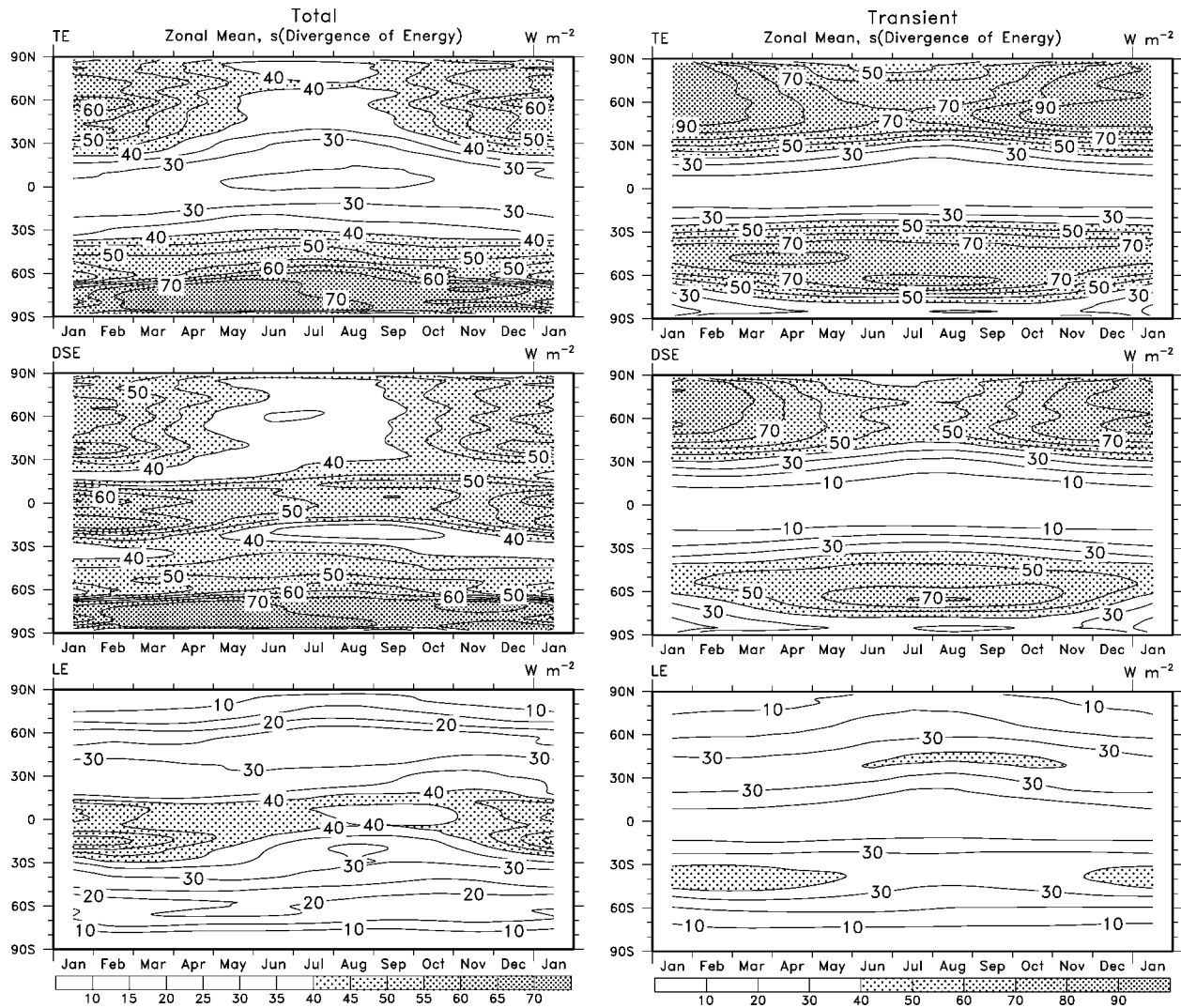
FIG. 11. Standard deviations of the total divergence of the zonal mean northward energy transport for 1979–2001 for the mean annual cycle, for the (top) TE, (middle) DSE, and (bottom) LE, for the total (left) and transients (right), with shadings given in the key. The units are \text{W m}^{-2} .
