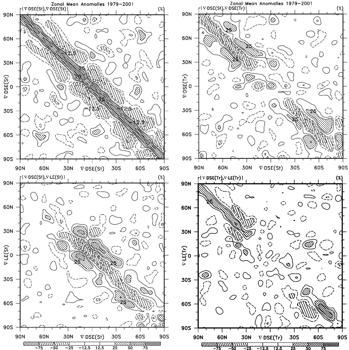
FIG. 12. Cross correlations of monthly transports of DSE (quasi-stationary) vs DSE (quasi-stationary), DSE (quasi-stationary) vs DSE (transient), DSE (quasi-stationary) vs LE (quasi-stationary), and DSE (transient) vs LE (transient). A contour of \pm 0.125 is plotted and beyond that the contour interval is 0.25, which is the 5% significance level if a degree of freedom is gained every 4 months (and hence is highly conservative).
