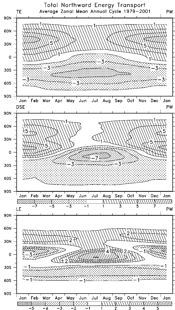
FIG. 3. Total zonal mean northward energy transport for 1979–2001 for the mean annual cycle, in PW. Shown are the atmospheric energy transports for the (top) TE, (middle) DSE, and (bottom) LE, with shadings given in the keys. The contour interval is 1 PW in the bottom panel but 2 PW in the top two panels.
