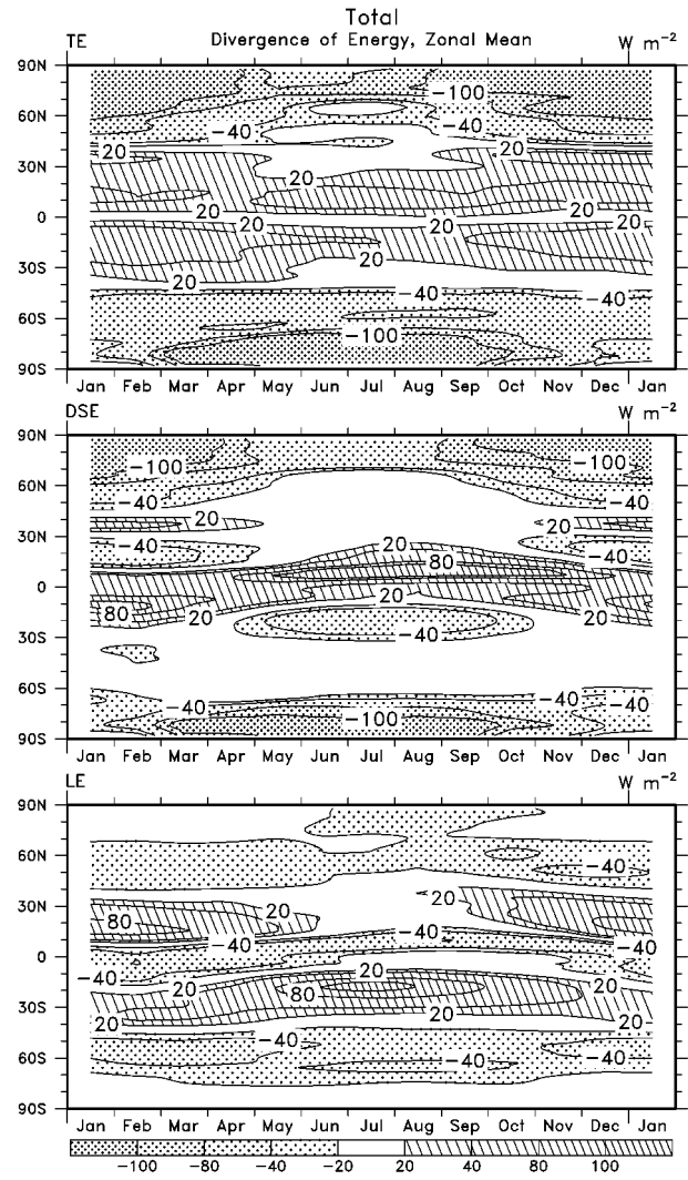
FIG. 5. Total divergence of zonal mean northward energy transport for 1979–2001 for the mean annual cycle, in W m^{-2} . Shown are the (top) TE, (middle) DSE, and (bottom) LE, with shadings given in the key. The contour interval is in the key.
