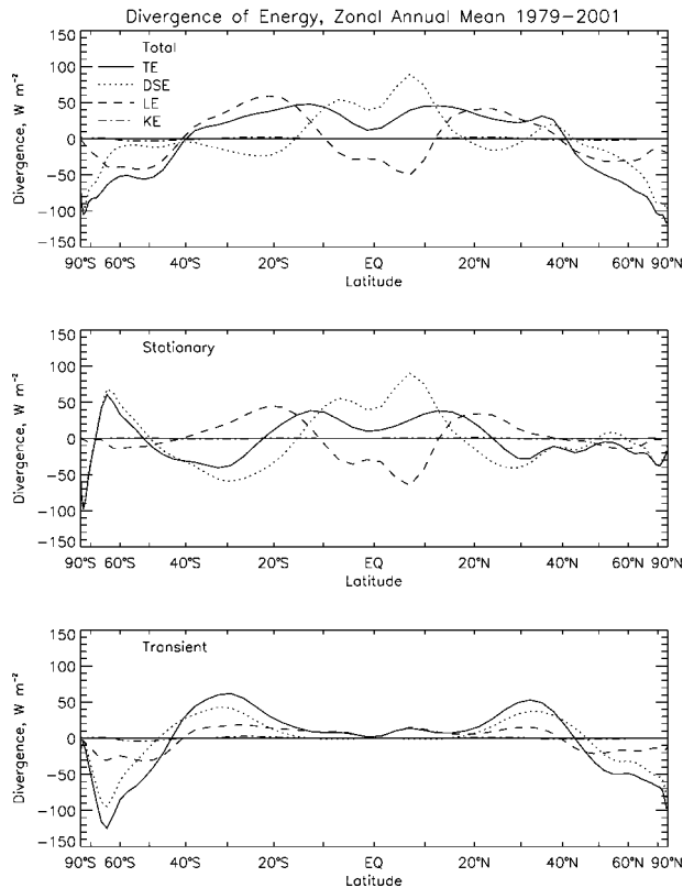
FIG. 2. Divergence of the annual mean for 1979–2001 northward energy transport zonally integrated for the (top) total atmospheric energy, (middle) quasi-stationary component, and (bottom) transient component, with the curves showing the total, dry static, and latent and kinetic energy components. Values are in \text{W m}^{-2} .
