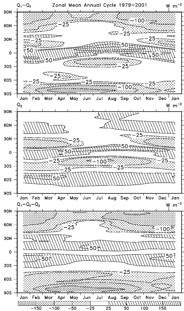
FIG. 7. Zonal mean heating components for 1979–2001 for the mean annual cycle, in W m^{-2} . Shown are the (top) diabatic heating Q_1 - Q_f , (middle) column latent heating Q_2 , and (bottom) total column atmospheric heating Q_1 - Q_f - Q_2 , with shadings given in the key. The contour interval varies but the same key applies to each panel.
