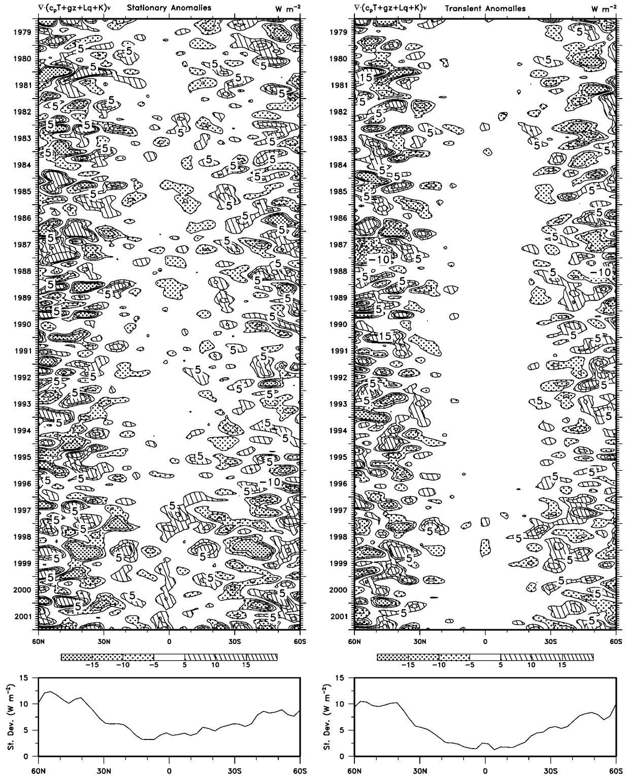
FIG. 9. Time series of zonal mean divergence of northward transport of TE for the (left) quasi-stationary and (right) transient components. The time series have been smoothed with a 1/12(1-3-4-3-1) filter that removes less than 3-month fluctuations. Units are W m^{-2} and shading as in the key.
