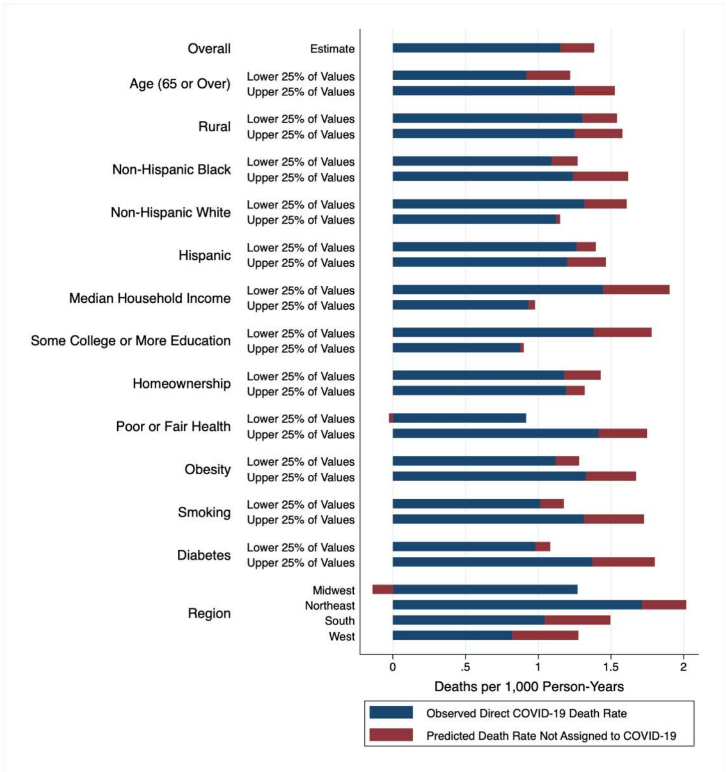
Fig 3. Decomposition of 2020 excess death rates across strata of sociodemographic and health factors a,b,c . a n = 2,096 counties. b Predicted death rates generated from primary model: M(i) = \alpha + \beta_1 M^*(i) + \beta_2 C(i) , where M(i) = Death rate from all causes in county i in 2020, M^*(i) = Death rate from all causes, county i in 2013–2018, and C(i) = COVID-19 death rate in county i in 2020. The model was weighted by the 2020 population and fully stratified into population-weighted quartiles for each sociodemographic or health factor. The death rates for the upper and lower 25% of values for each factor are presented in this figure. c Indirectly age-standardized death rates are presented in S4 Fig . COVID-19, Coronavirus Disease 2019.
