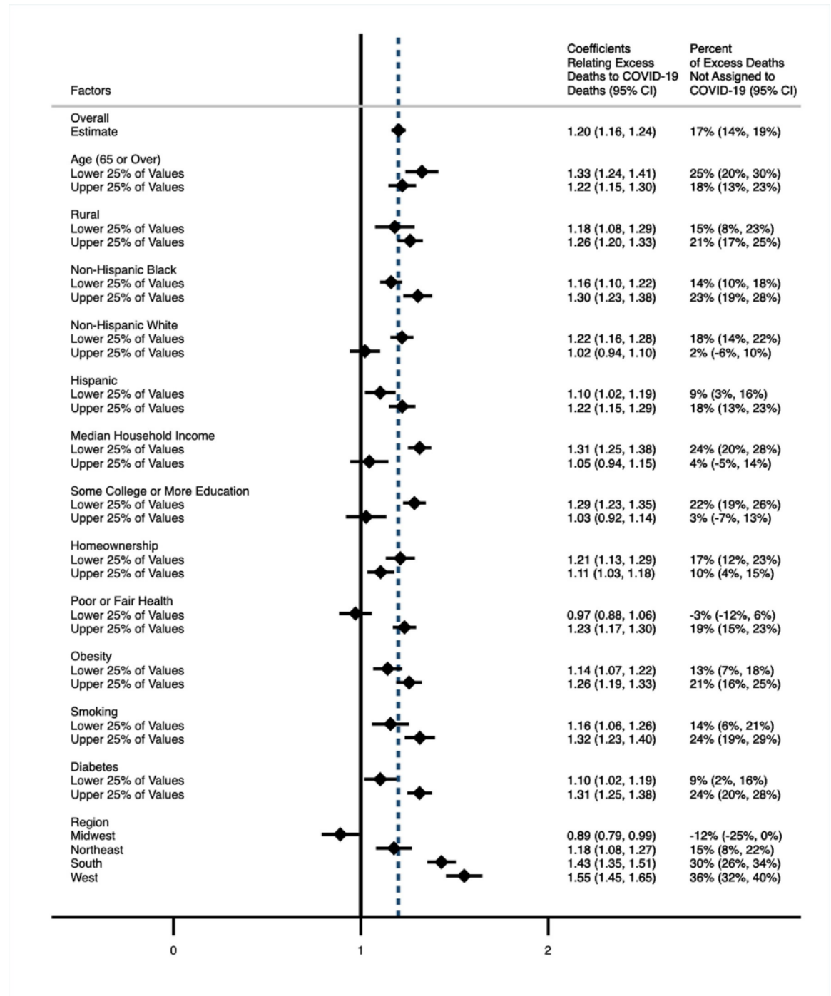
Fig 2. Relationship between all-cause mortality and direct COVID-19 mortality across strata of sociodemographic and health factors a,b,c,d,e . a n = 2,096 counties. b \beta_2 coefficients generated from primary model: M(i) = \alpha + \beta_1 M^*(i) + \beta_2 C(i) , where M(i) = Death rate from all causes in county i in 2020, M^*(i) = Death rate from all causes, county i in 2013–2018, and C(i) = COVID-19 death rate in county i in 2020. The model was weighted by the 2020 population and fully stratified into population-weighted quartiles for each sociodemographic or health factor. The coefficients for the upper and lower 25% of values for each factor are presented in this figure. c Sample interpretation: In counties with lower household income, for every 1 directly assigned COVID-19 death, there was an increase in 1.31 all-cause deaths, suggesting there were 0.31 deaths not assigned to COVID-19 for every 1 directly assigned COVID-19 death in these counties. d Indirectly age-standardized models are presented in S3 Fig . e The dashed line represents the overall estimate. The solid line represents a coefficient of 1, which indicates that for every 1 directly assigned COVID-19 deaths, 0 deaths not assigned to COVID-19 occurred. COVID-19, Coronavirus Disease 2019.
