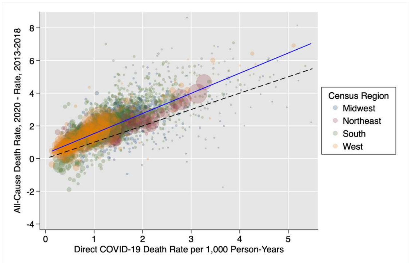
Fig 1. Difference between the 2020 all-cause mortality rate and 2013–2018 historical mortality rate vs. 2020 direct COVID-19 mortality rate ( n = 2,096 ) a,b,c . a The solid blue line represents a linear model of best fit weighted by population size. b The dashed reference line represents a slope of 1. c Six counties with a direct COVID-19 death rate greater than 6 deaths per 1,000 person-years or a difference between 2020 all-cause and 2013–2018 all-cause death rates greater than 10 deaths per 1,000 person-years were excluded from the figure for the purpose of visualization. These counties were included in all regressions. COVID-19, Coronavirus Disease 2019.
