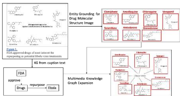
Figure 6: Expanding KG through Subfigure Segmentation and Cross-modal Entity Grounding. The figure image shown here is from (Ekins and Coffee, 2015)
