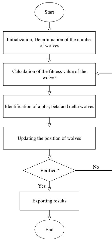
Figure 4. GWO algorithm
