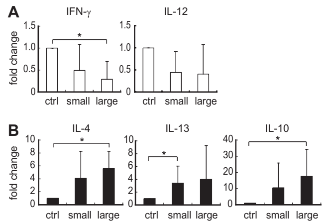
Fig. 2. Apc Min/+ mouse polyps showed a Th2-predominant tumor microenvironment. (A and B) qRT-PCR analysis was performed for cytokine milieu in Apc Min/+ mouse polyps. Histologically normal mucosa was used as control (ctrl) ( n = 6). * P < 0.05. (A) Th1 cytokines (IFN- \gamma and IL-12) were suppressed in Apc Min/+ mouse polyps in a polyp size-dependent manner. (B) Th2 cytokines (IL-4, IL-13 and IL-10) were upregulated in Apc Min/+ mouse polyps in a polyp size-dependent manner.
