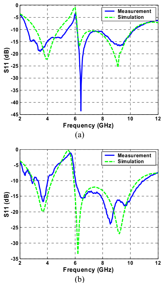
Fig. 3. Measured and simulated return loss (a) U-shaped slot (b) C-shaped slot
