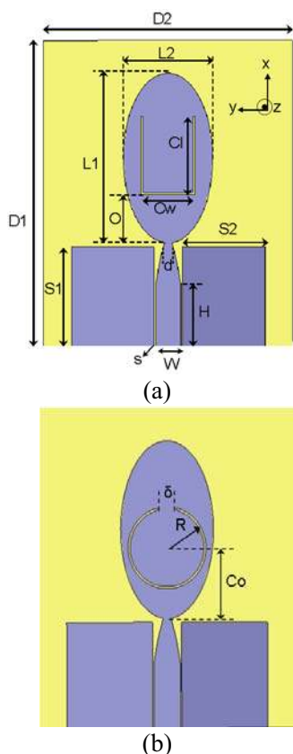
Fig. 2. Elliptical monopole schematic with (a) U-shaped slot (b) C-shaped slot
