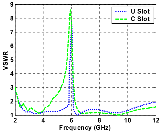
Fig. 4. VSWR measurement
