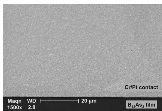
FIG. 5. SEM image of the Cr/Pt (50/100 nm) contact after annealing at 600 °C for 30 s in UHP Ar. The edge of the patterned contact is shown at the bottom of the image.
