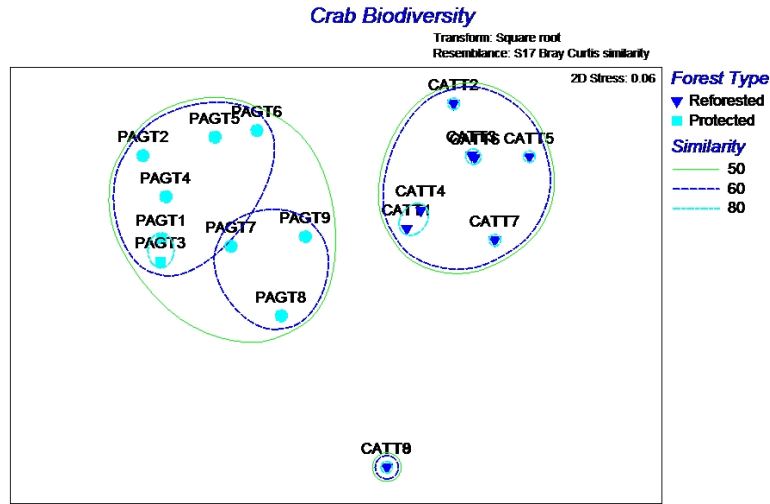
Fig. 4: NMDS plots of crab densities sampled from reforested and protected mangrove forests. Sites clustered into two groups at the 50% similarity level and three groups at the 60% level
