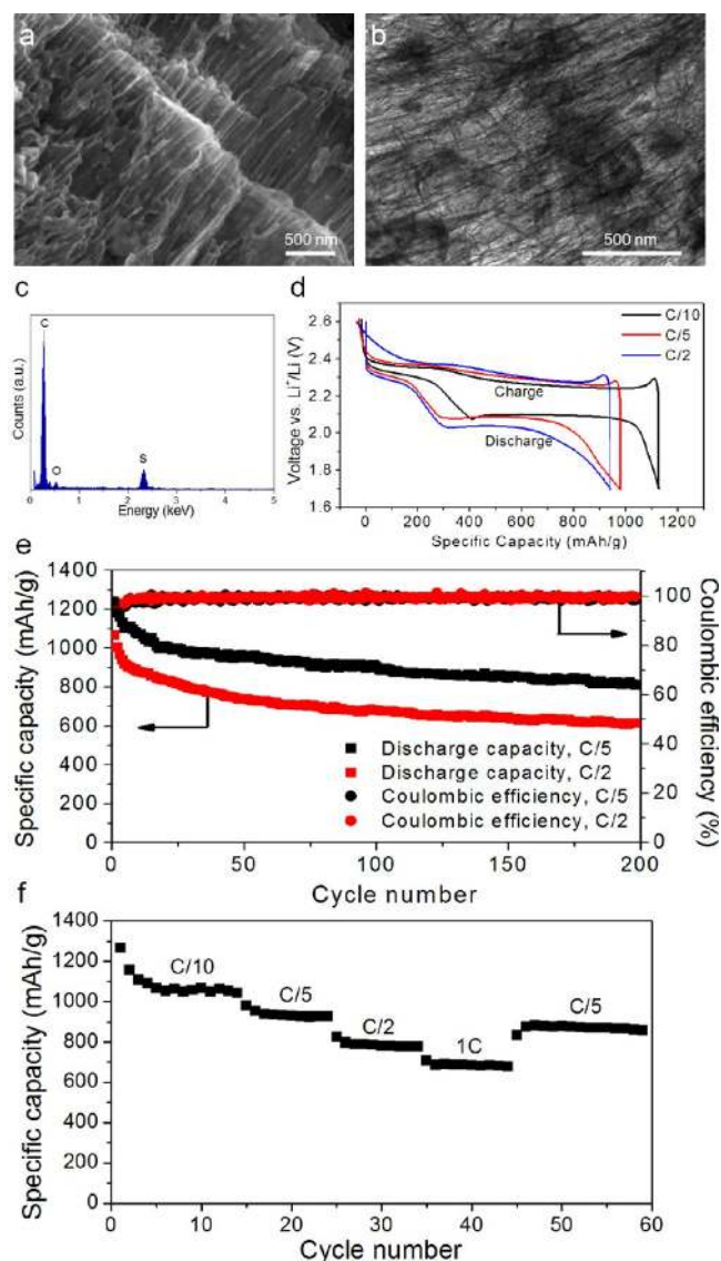
Figure 4. Nanostructures and electrochemical performance of sulfur encapsulated by crab shell-templated carbon as Li-ion battery electrode. (a and b) SEM and TEM images of sulfur encapsulated by crab shell-templated carbon showing nanochannel array structures. (c) EDX spectrum indicating the presence of sulfur and carbon without other impurities. (d) Typical discharge/charge voltage profiles of the sulfur electrode at C/10, C/5, and C/2 rates. (e) Capacity and Coulombic efficiency at C/5 and C/2 versus cycle number. (f) Rate capabilities on discharge of the crab shell-templated sulfur electrode.
