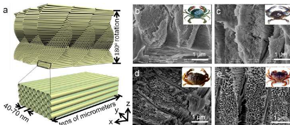
Figure 1. Structural model and SEM images of crab shell templates. (a) Structural model of twisted plywood nanochannel arrays in crab shell templates showing the hollow channels created by removing organic nanofibers in crab shells. The hollow channels are arranged parallel to each other to form horizontal planes stacked in a helicoid fashion, creating a twisted plywood structure. (b–e) SEM images of the biotemplates from a Chinese hairy crab shell, a blue crab, a stone crab, and a Dungeness crab, respectively, demonstrating the universal nature of the nanochannel arrays in crab shell templates.
