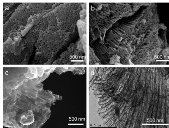
Figure 3. SEM and TEM characterization to show the preservation of nanochannel arrays during the carbon coating process. (a–c) SEM images of polydopamine-coated crab shell template, carbon-coated crab shell template, and carbon nanochannel arrays after removing the CaCO 3 framework, respectively. (d) TEM image of carbon nanochannel arrays after removing the CaCO 3 framework.
