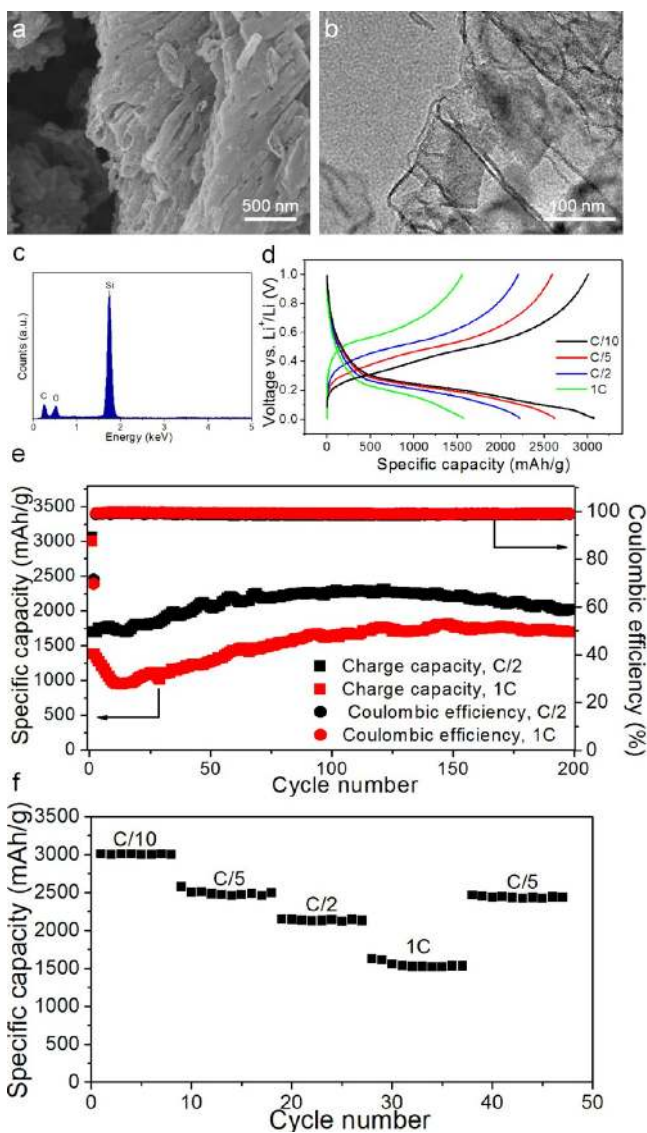
Figure 5. Nanostructures and electrochemical performance of silicon encapsulated in crab shell-templated carbon for Li-ion battery electrodes. (a and b) SEM and TEM images showing the nanochannel array structure. (c) EDX spectrum indicating the presence of carbon and silicon. (d) Typical discharge/charge voltage profiles at C/10, C/5, C/2, and 1C rates. (e) Reversible capacity and Coulombic efficiency at C/2 and 1C versus cycle number. The cells were activated with a slower rate on the first cycle (C/10). (f) Rate capabilities of the electrode.
