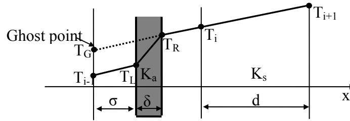
Figure 1. 1-D 'ghost point' finite difference heat diffusion model. Heat flux is balanced when it flows into, through and out of the crack.
