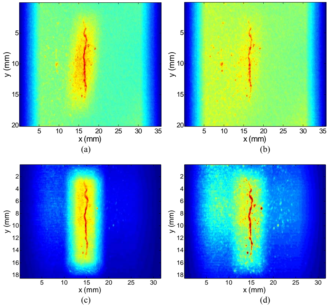
Figure 17. Titanium test-piece with a crack of 11mm long, 3 \mu m wide. (a) Summed first derivative imaging result by LLT method; (b) Summed second derivative imaging result using the LLT method; (c) Summed first derivative imaging result by the LST method (d) Summed second derivative imaging result by the LST method.
