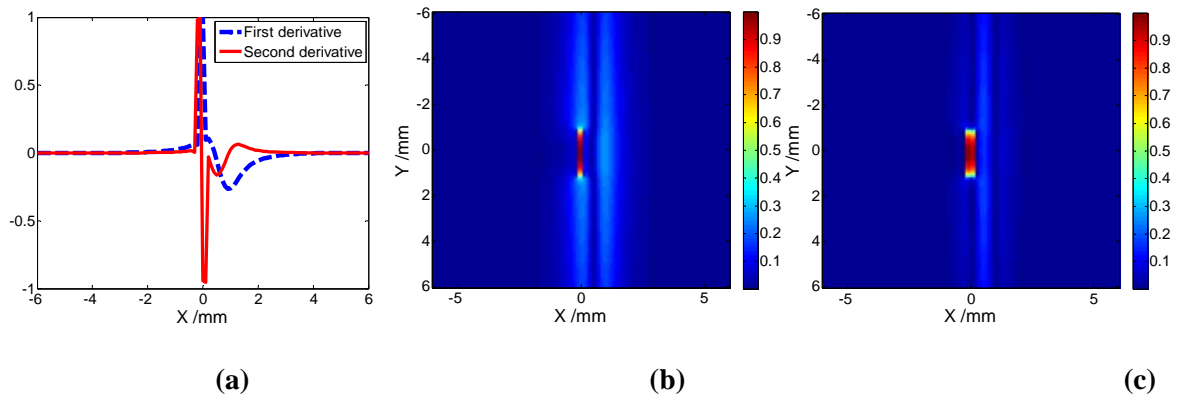
Figure 7. (a) Normalized first (blue line) and second (red line) spatial derivatives of the temperature profile line in figure 5a. (b) First derivative image, in the x -direction, of figure 5a image. (c) Second derivative image, in the x -direction, of the image in Figure 5a.
