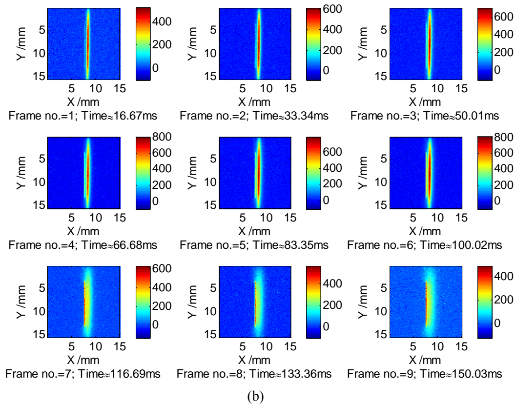
Figure 15. (a) Experimental laser line thermal images of a crack of 10mm length, 2mm depth and 50 \mu m width in a stainless steel plate. (b) Corresponding simulated thermal images.
