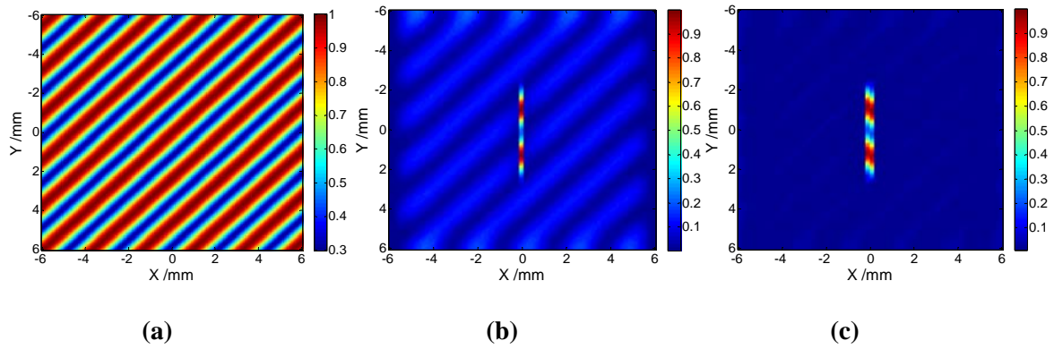
Figure 12. Laser line source scans across the block using a 2x laser beam radius step length. (a) Simulations of thermal images of the laser line at each scan position. (b) Cumulative first differential image. (c) Cumulative second differential image.
