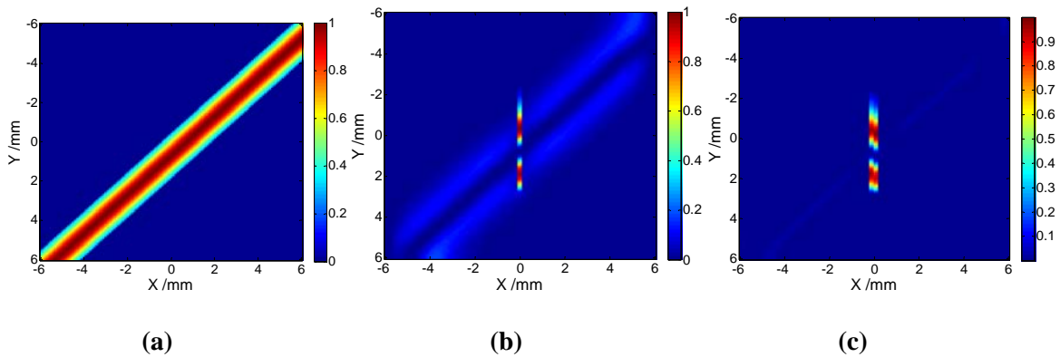
Figure 11. Laser line source crossing the centre part of the crack. (a) Simulation of thermal image of the laser line (b) First differential image. (c). Second differential image.
