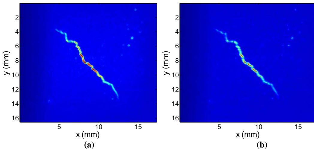
Figure 16. (a) Summed first derivative thermal images of a crack using the laser line source. (b) Summed second derivative thermal image.
