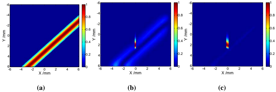
Figure 10. Laser line source crossing the tip of the crack. (a) Simulation of thermal image of the laser line (b) First differential image. (c). Second differential image.
