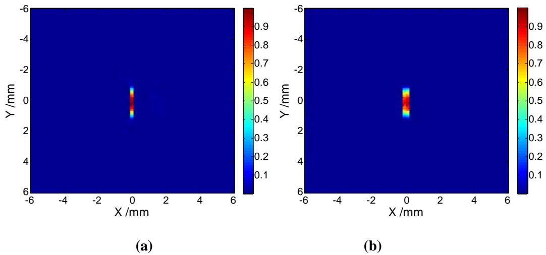
Figure 8. (a) Summed first derivative image in the x -direction from 0.1s to 0.3s. (b) Summed second derivative images in the x -direction from 0.1s to 0.3s. The noise level was \pm 0.1K .
