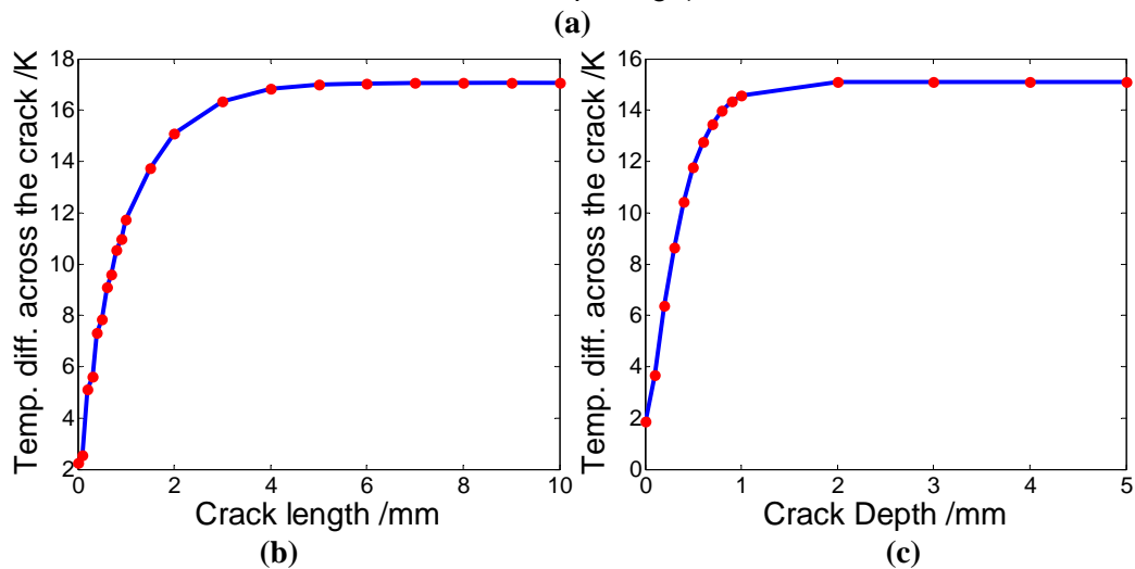
Figure 6. Temperature difference across a crack for a laser line source when (a) crack opening changes. (b) crack length changes. (c) crack depth changes.
