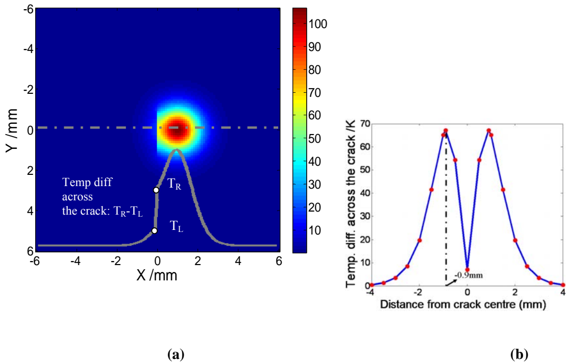
Figure 4. (a) Simulation of laser spot image after 50ms heating. (b) Temperature difference across the crack as a function of laser spot distance to the crack.
