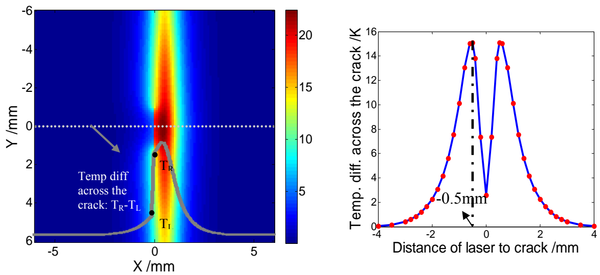
Figure 4. (a) Simulation of laser spot image after 50ms heating. (b) Temperature difference across the crack as a function of laser spot distance to the crack.
