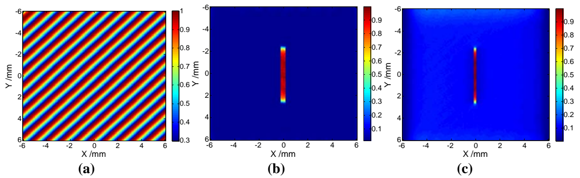
Figure 13. Laser line source scans across the block using a 1x laser beam radius step length. (a) Simulations of thermal images of the laser line at each scan position. (b) Cumulative first differential image. (c) Cumulative second differential image.
