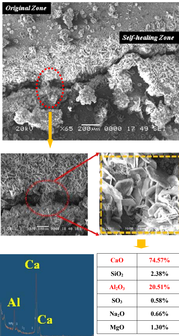
Fig. 14 Self-healed re-hydration products in crack by hydrogarnet phases (C-A-H) and calcite phases (CaCO 3 ) in case of sample II.
