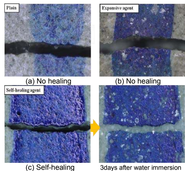
Fig. 24 Self-healing behaviour of cementitious composite materials incorporating geo-materials [Water/Binder ratio = 0.45].
