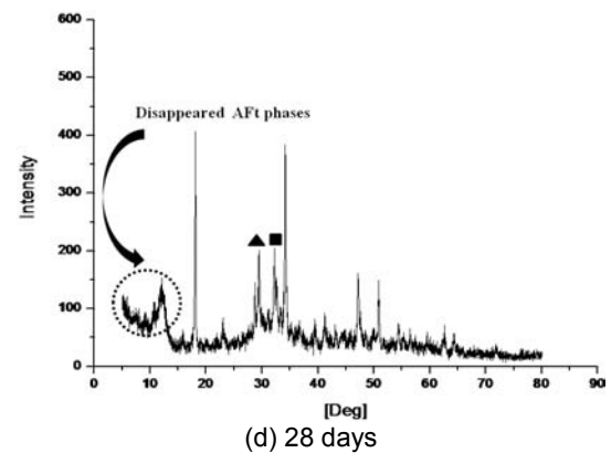
Fig. 7 Main hydration products of sample I [OPC 90% + CSA 5% + Geo-materials 5%] pastes at normal water/binder ratio of 0.45 (the three-component system).
