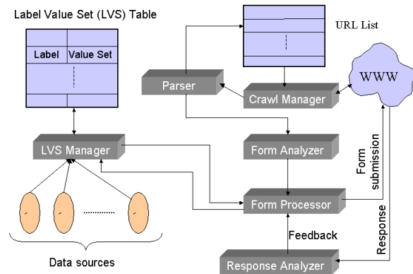
Figure 1: HiWE Architecture
