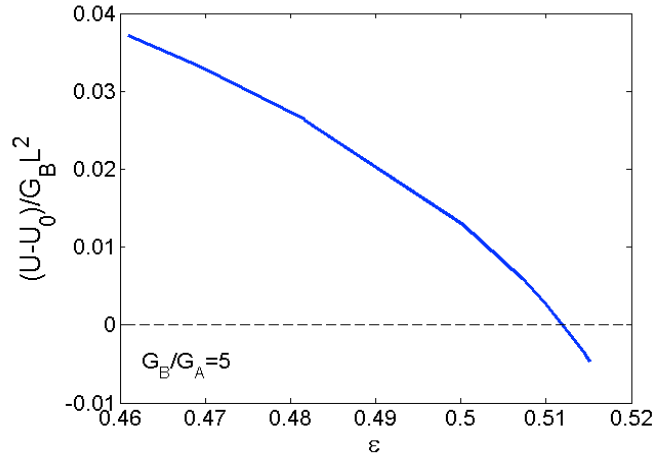
Fig. 2. The energy difference between the creased state U and the flat state U_0 plotted as a function of the applied strain \epsilon for a fixed value of the modulus ratio G_B/G_A = 5 . When \epsilon = 0.512 , the energy of the creased state is equal to the energy of the flat state, and \epsilon = 0.512 is identified as the critical condition for the onset of interfacial creases.
