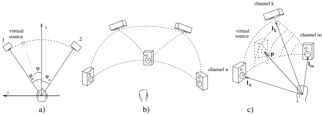
Figure 1: a) A standard stereophonic listening configuration. The virtual source can be positioned between the loudspeakers. b) A 3-D loudspeaker configuration is divided to loudspeaker triangles. c) The standard stereophonic listening configuration being extended with third loudspeaker. The listener perceives a virtual source that is located inside the triangle.
