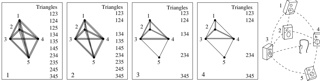
Figure 2: Initial triangularization process for five loudspeakers in 3-D setup. Step 1 : All triangles are formed. Step 2 : Too narrow triangles are removed. Step 3 : Crossing sides are resolved. Step 4 : Triangles that include loudspeakers are removed. The result of the process is seen in the rightmost figure.
