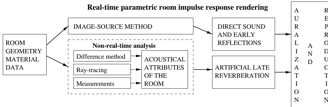
Figure 4: A parametric room impulse response rendering method used in DIVA system
