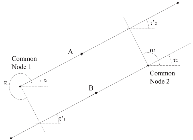
Fig. 8. Example of a scheme of the angles considered in the determination of the lateral type of topology (right-left).
