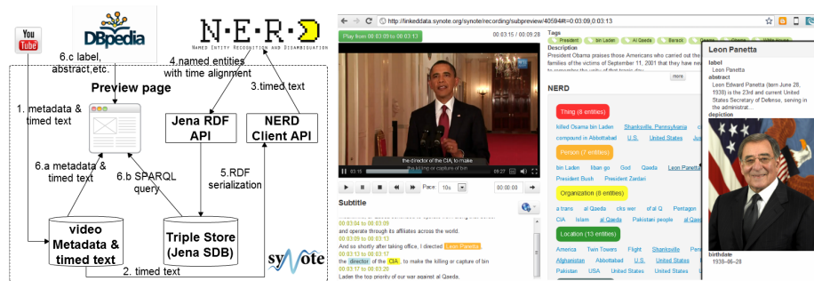
Fig. 1. a) Synote and NERD integration architecture. b) The Synote UI enriched with NERD and DBpedia.
