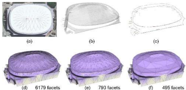
Fig. 10 Simplification of the mesh patches on an irregular roof- (a) an aerial picture of the scene, (b) the input point set with a 17 pts/m 2 density, (c) the extracted 3D-line segments, and the obtained 3D-models with (d) fine, (e) medium and (f) coarse mesh-patches. Note that the primitive arrangement and the facades are not affected by the simplification process.
