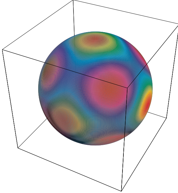
FIG. 1: A density plot of the function \mathcal{P}_\Phi(\hat{k}) for n = 3/2 .
