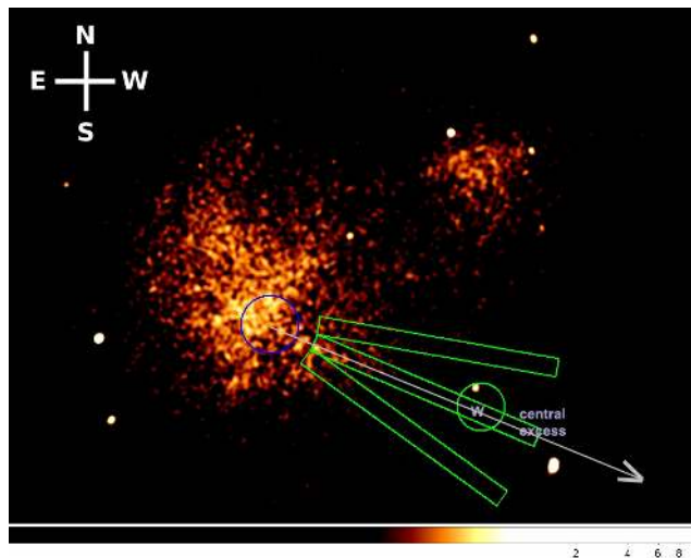
Figure 7. Chandra ACIS-S3 X-ray image of Abell 2744, smoothed with a 3 pixel kernel Gaussian. We analyse the cluster’s X-ray profile in three rectangular regions, each 150'' in length and radiating from the cluster centre (marked by the blue circle). We find marginally significant excess X-ray emission in the central rectangular region, which extends towards the Western clump (marked by the green circle).
