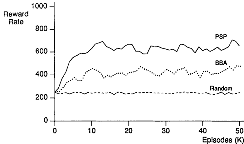
Figure 5. Performance profiles of systems using different credit assignment methods.
