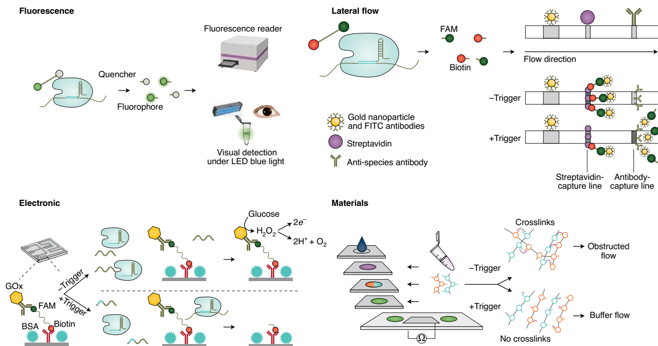
Fig. 4 | Collateral-cleavage readouts. Top left: fluorescence readouts rely on quenched fluorophores that, on target recognition, are released as a result of the collateral cleavage of the DNA or RNA oligomers joining the fluorophore and quencher. The signal can be measured by a fluorescence reader or read by eye under blue light. LED, light-emitting diode. Top right: lateral-flow-based immunochromatographic readouts rely on the high affinity of streptavidin and biotin, and use a reporter molecule consisting of a DNA or RNA oligomer conjugated to FAM and biotin. The product of the CRISPR reaction is deposited on the sample-application area of a test strip, at which point FAM binds to gold-nanoparticle-labelled FITC-specific antibodies. When intact, the reporter oligomer remains bound to the streptavidin line through biotin, creating one colour band on the test strip. When the reporter oligomer is cleaved, FAM and the bound gold-labelled FITC-specific antibodies flow farther on the strip and bind to secondary anti-species antibodies, which leads to the formation of a second colour band. Bottom left: electrochemical readout relying on the amperometric detection of \text{H}_2\text{O}_2 in an electrochemical cell 46 . Anti-fluorescein antibodies (green) coupled with glucose oxidase (GOx) bind to FAM-carrying RNA reporter molecules, which are immobilized through biotin on a surface. The concentration of GOx is reduced in the presence of an RNA trigger, owing to the activated crRNA/Cas13a complex cleaving the RNA reporter molecule on target recognition, which frees the GOx-carrying anti-fluorescein antibodies from the surface. Bottom right: in the presence of a dsDNA trigger, Cas12a collaterally cleaves ssDNA linkers within a hydrogel. This prevents crosslinking within the hydrogel, thereby modulating the permeability of a paper-based microfluidic device and allowing for buffer flow, which can be measured electrically 79,80 .
