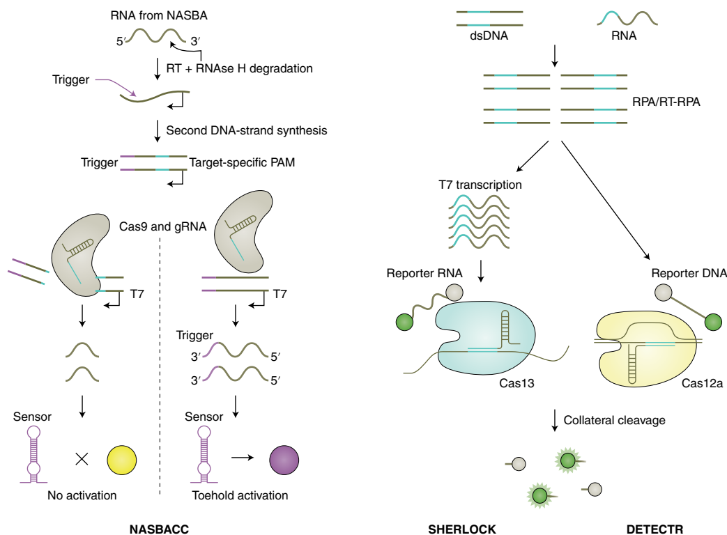
Fig. 1 | Two strategies for CRISPR-based diagnostics. Left: RNA targets are amplified through NASBA, which starts with reverse transcription (RT) to complementary DNA using a sequence-specific primer that appends a trigger sequence (magenta) to the toehold sensor. The RNA from the RNA/DNA hybrid is destroyed by RNase H, enabling a primer that contains a T7 promoter to bind and create a complementary second DNA strand. T7 transcription of the dsDNA template creates the target RNA sequence, which can be used as starting material for a new NASBA cycle or detected by the toehold sensor. If a PAM sequence (blue) is present in the dsDNA amplicon, Cas9-mediated cleavage leads to a truncated template for T7 transcription, which generates a shorter target RNA that cannot activate the toehold sensor. In the absence of the PAM sequence, a full-length target RNA containing the trigger is transcribed, which activates the toehold sensor and produces a visible change in colour. Right: DNA or RNA are amplified by RPA or RT-RPA, respectively. For RNA-targeting CRISPR enzymes (including Cas13a), the amplified RPA product is T7-transcribed into RNA. Binding of the crRNA to the complementary target sequence activates the Cas enzyme and triggers collateral cleavage of quenched fluorescent reporters. Thereby, Cas13a (used in SHERLOCK) or Cas12a (used in DETECTR) indicate the presence of RNA or DNA target sequences, respectively.
