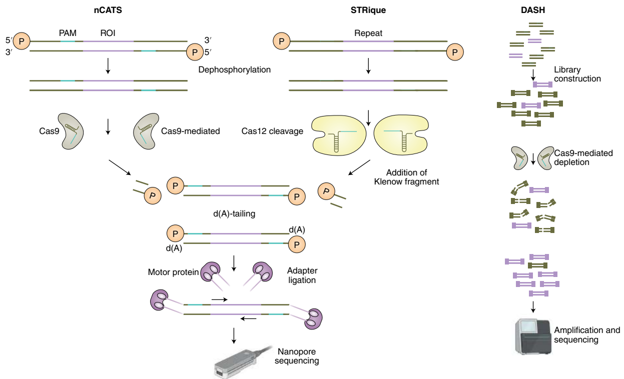
Fig. 3 | CRISPR-Cas-mediated enrichment strategies for sequencing-based diagnostics. Left: nCATS is a Cas9-based enrichment technology, which first dephosphorylates DNA ends and then uses Cas9 to induce cuts near a region of interest (ROI) that contains a PAM sequence. A DNA polymerase I with an N-terminal truncation that lacks exonuclease activity (Klenow fragment) enables the addition of dAMP (deoxyadenosine monophosphate (dA)) to the 3' end the DNA fragment (d(A)-tailing)). Next, adapters containing a motor protein are ligated to the DNA at Cas9 cleavage sites, enabling the DNA to pass through the nanopore. STRique uses Cas12a for the enrichment of repeat-containing regions analysed by nanopore sequencing, and employs an algorithm for the identification of the position of the repeat flanking regions and the number of repeats. Right: DASH uses Cas9 to deplete unwanted sequences (black) before next-generation sequencing. Non-targeted sequences (magenta) retain intact adapters for amplification and sequencing.
