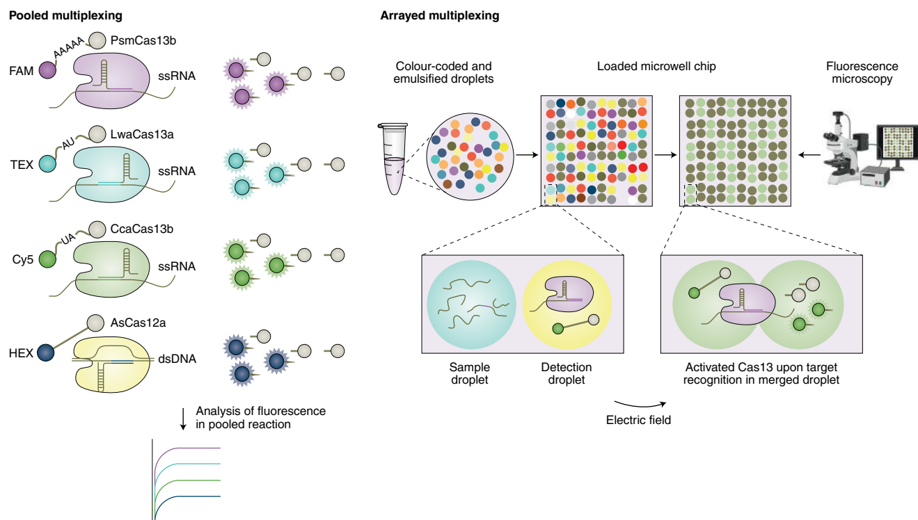
Fig. 2 | Multiplexed CRISPR-based target detection. Left: pooled multiplexing of up to four targets, as implemented in SHERLOCKv2. Orthogonal CRISPR enzymes (PsmCas13b, LwaCas13a, CcaCas13b, AsCas12a), each cleaving preferentially different reporter molecules bearing different fluorophores (FAM, TEX615 (TEX), Cy5, hexachlorofluorescein (HEX)) with distinct absorbance and emission wavelengths. Right: in CARMEN, a distinct colour code is added to each PCR-amplified sample or Cas13-based detection mix. The Cas13-based detection mix contains Cas13a, a sequence-specific crRNA and a cleavage reporter. The colour-coded solutions are emulsified in fluoros oil, which creates nanolitre droplets. Droplets from all samples and detection mixes are pooled together and loaded into a microwell-array chip in one step to create all possible pairwise combinations. The droplet pair in each well is identified using fluorescence microscopy before they are merged by exposure to an electric field. Fluorescence microscopy is then used to monitor each Cas13-based detection reaction.
