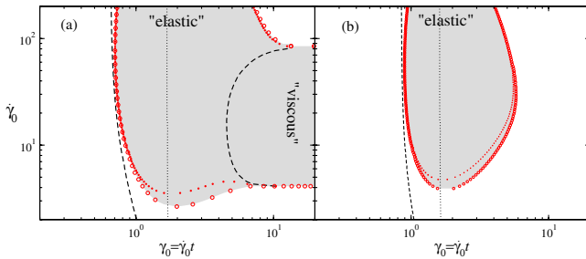
FIG. 4 (color online). Shear startup in the Rolie-Poly model. Unstable region shaded. (a) Nonmonotonic constitutive curve, \beta = 0.4 , \tau_R = 0.0 , \eta = 10^{-4} . Large circles: Full onset criterion. Right dashed line delimits viscous criterion (11). Left dashed line: Elastic criterion (12). Small circles: Elastic plus viscous terms (12) + (11). Dotted line: stress overshoot \partial_{\dot{\gamma}_0} \Sigma_0 = 0 . (b) Corresponding figure for monotonic constitutive curve, \beta = 1.0 .
