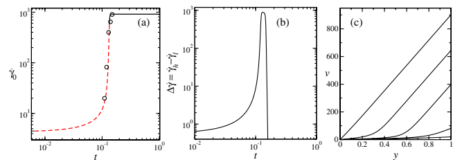
FIG. 1 (color online). Nonstretch RP model: \beta = 0.8 , \eta = 10^{-4} , \Sigma_0 = 0.7 . (a) Time derivative of creep curve. Dashed line: linearly unstable regime. (b) Corresponding degree of banding (difference in maximum and minimum shear rate across cell). (c) Flow profiles at times marked by circles in (a) for \epsilon_n = 0.1\delta_{n,1} , l = 10^{-2} .
