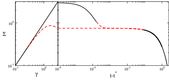
FIG. 3 (color online). Left: Stress vs strain for a fast ramp in the RP model. \beta = 0.0 , \tau_R = 10^{-4} , \eta = 10^{-5} . Right: Relaxation postramp; unstable region in a dashed line. Upper curve: Appreciable chain stretch, \tau_R \dot{\gamma} \rightarrow \infty . Lower: Negligible stretch, \tau_R \dot{\gamma} = 0.1 .
