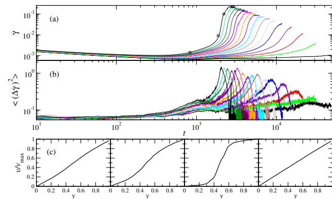
FIG. 2 (color online). SGR model: (a) Differentiated creep curves for stress values \Sigma_0/\Sigma_y = 1.005, 1.010, \dots, 1.080 (curves upwards). (b) Corresponding degree of banding. (c) Normalized velocity profiles for the circles in (a). x = 0.3 , w = 0.05 , n = 50 , m = 10000 . Initial sample age t_w = 10^3[1 + \epsilon \cos(2\pi y)] , \epsilon = 0.1 .
