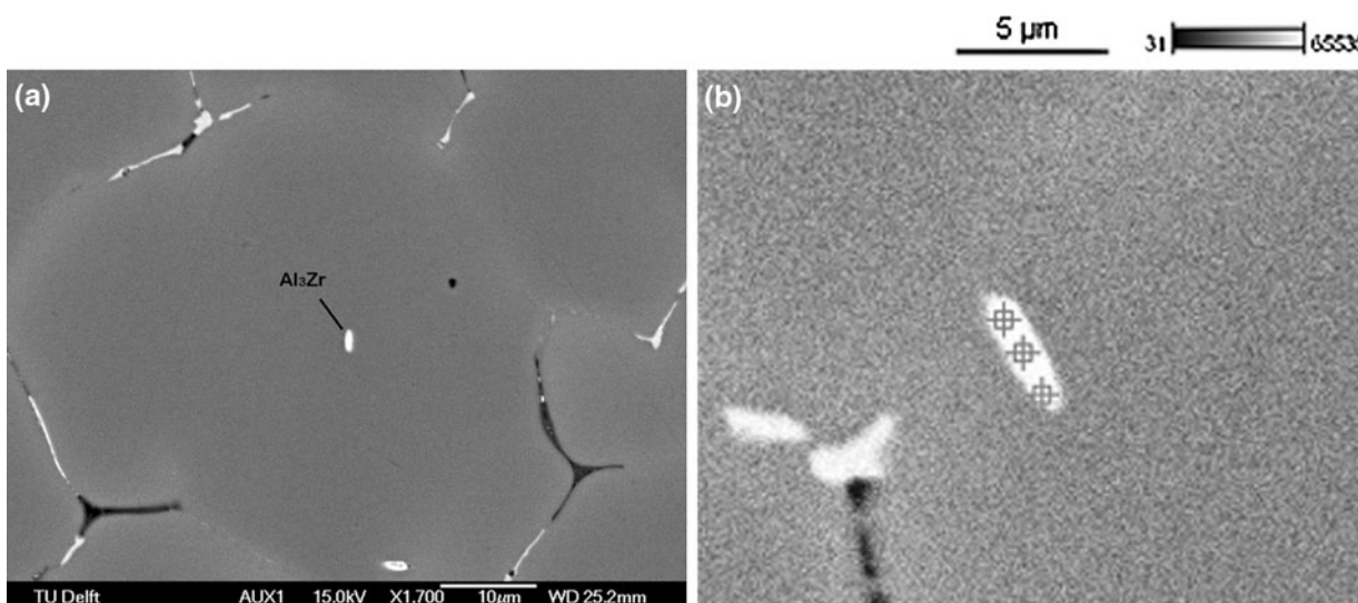
Fig. 8—Intermetallics found in an aluminum alloy with 0.6 mass pct Zr and 0.06 mass pct Ti after ultrasonic treatment at 710 °C: (a) general view (white particle in the center) and (b) Al 3 Zr particle at a higher magnification.
