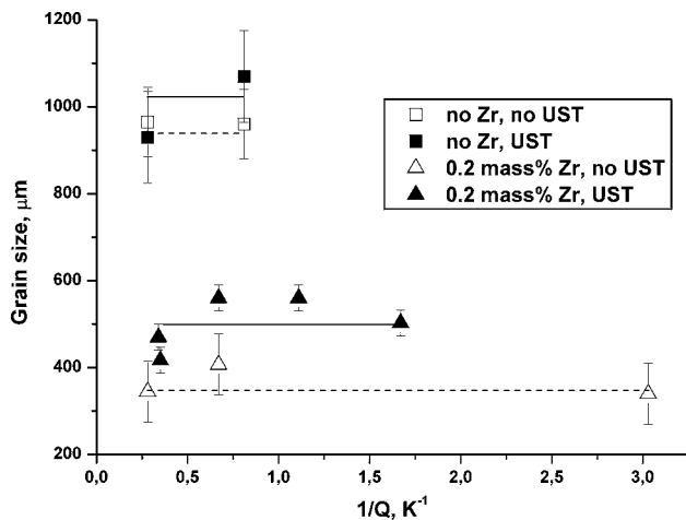
Fig. 10—Relationship between the grain size and inverse growth restriction factor in Al-Zr-V alloys. Growth restriction factor Q is calculated from the V concentration in the alloys.
