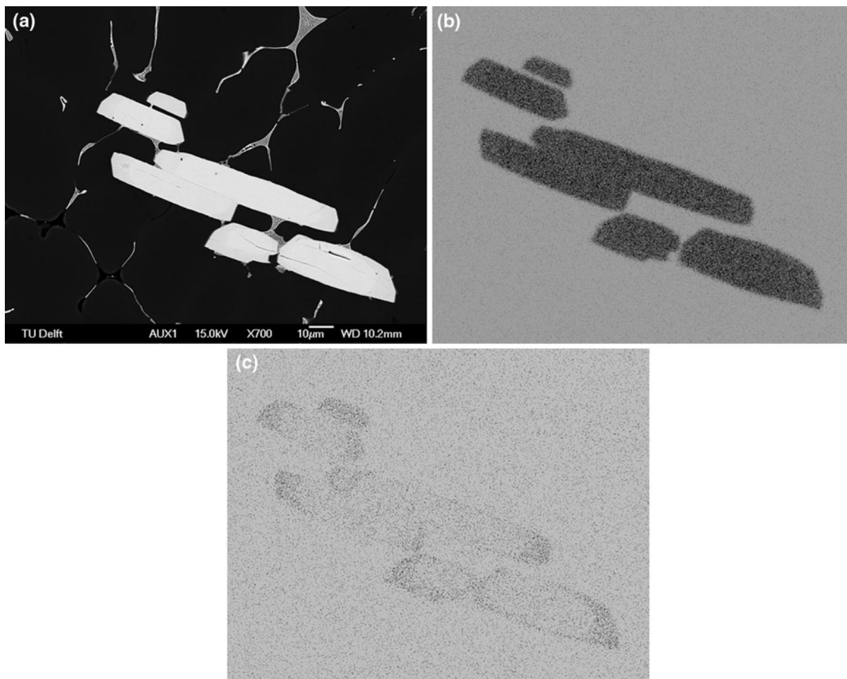
Fig. 7—Intermetallics found in an aluminum alloy with 0.6 mass pct Zr and 0.06 mass pct Ti cast without ultrasonic treatment: (a) general view, note slightly different contrast at the edges of the plates; (b) EDS mapping of Zr concentration; and (c) EDS mapping of Ti concentration.
