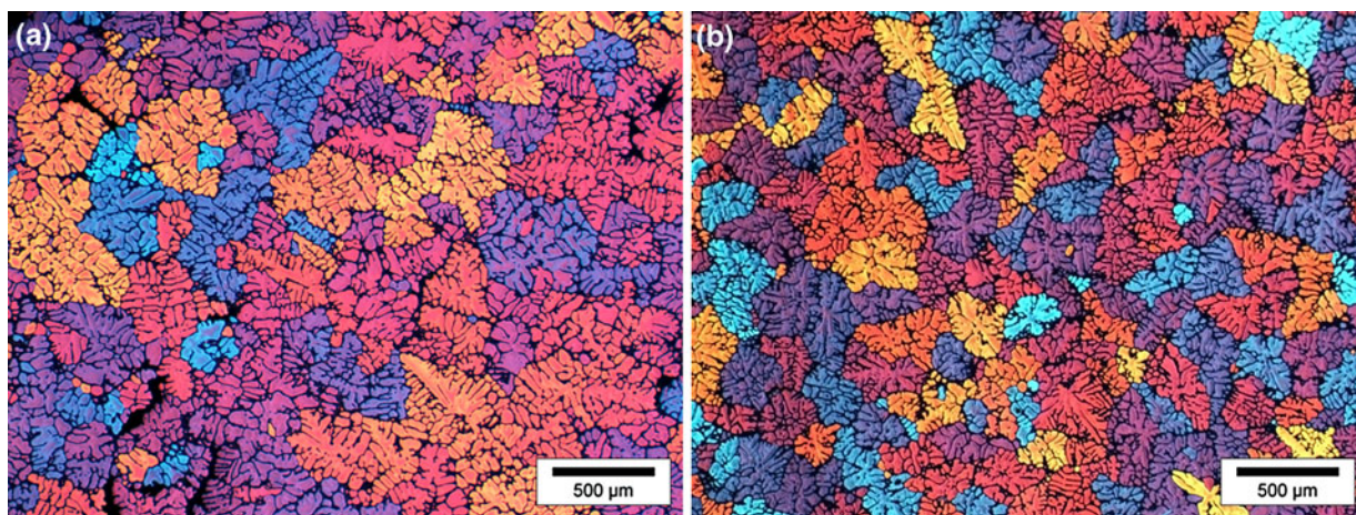
Fig. 4—Effect of UST during 10 s in the liquid state on the grain size and morphology of an Al-11 mass pct Cu alloy: (a) without UST in the presence of immersed idle ultrasonic horn and (b) after UST.
