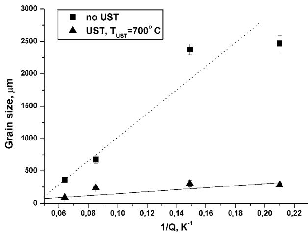
Fig. 9—A re-plot of Fig. 5 showing the relationship between the grain size and inverse growth restriction factor in Al-Zr-Ti alloys. Growth restriction factor Q is calculated from the Ti concentration in the alloys.
