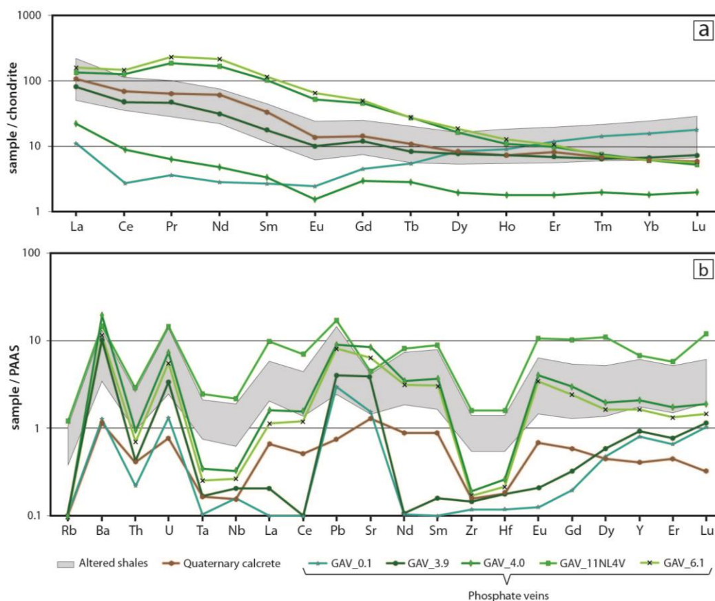
Figure 8. (a) REE plots of Llandoverian shales, Quaternary calcrite and supergene phosphate mineralisations of the Gavà weathering profile normalised to chondrite C1 (McDonough and Sun, 1995); (b) Multi-element trace element composition of the same lithologies normalised to the Post Archaean Australian Shales (PAAS; [45]).
