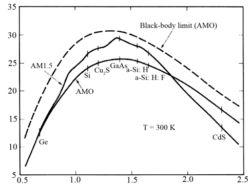
Figure 5. Dependency of the conversion efficiency on the semiconductor band gap [3]
