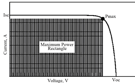
Figure 6. The I-V characteristic of an ideal solar cell [15]
