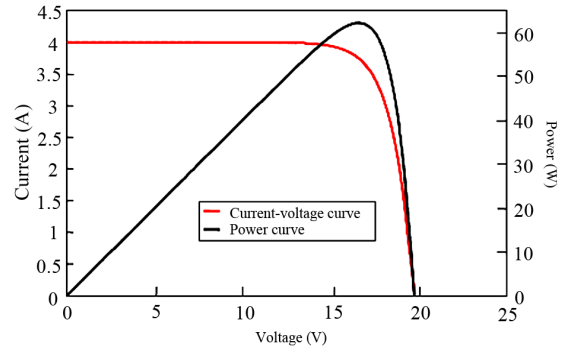
Figure 3. Typical I-V characteristic of a crystalline silicon module with the variation of power [7]
