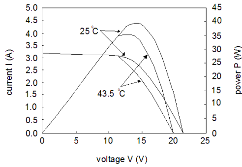
Figure 4. I-V and P-V characteristics of solar cell module [9]
