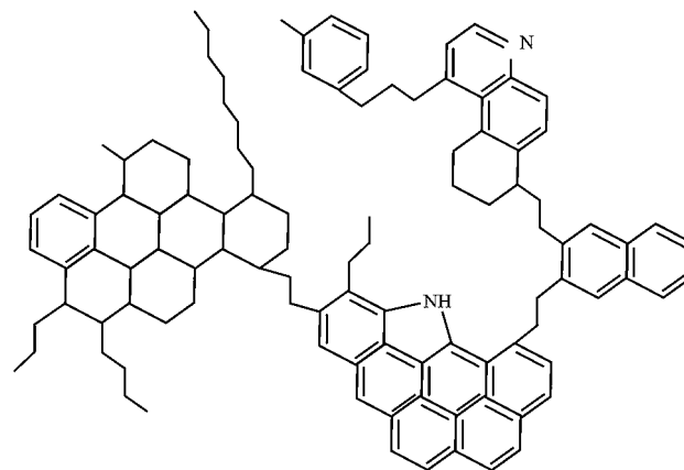
Fig. 4 Molecular structure of an asphaltene (Groenzin and Mullins 2000)
