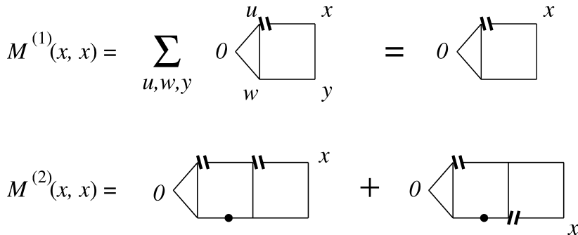
FIG. 8. The one-loop and two-loop diagrams for lattice animals. Lines ending with double bars represent \tilde{\rho}_p^a -lines.
