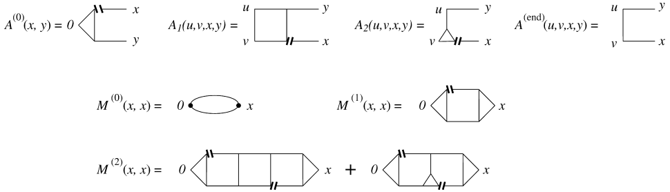
FIG. 9. The diagrams for percolation. Lines ending with double bars represent \tilde{\tau}^a -lines.
