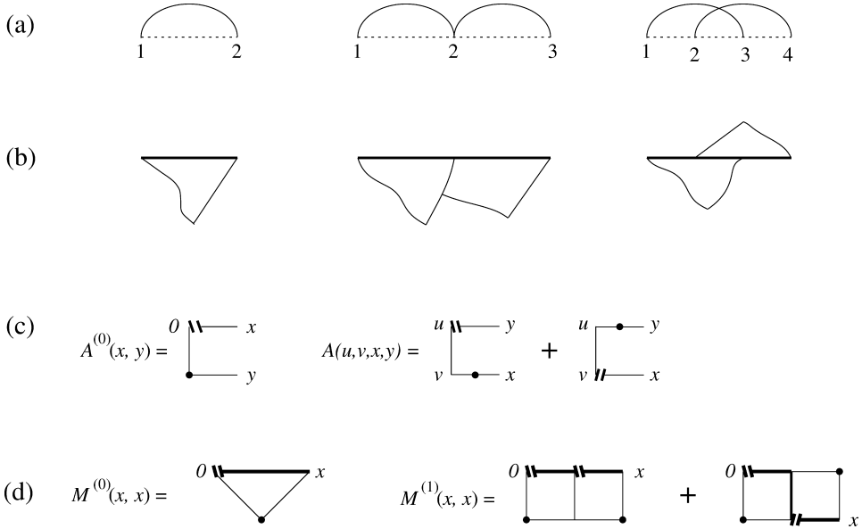
FIG. 6. (a) The laces with one and two edges. (b) Bead intersections imposed by the laces. (c) Constituents for constructing M^{(N)} , where A stands for both A^{(i)} and A^{(\text{end})} . Lines ending with double bars represent \tilde{\rho} -lines. (d) The one-loop and two-loop lattice tree diagrams, with lines corresponding to the backbone drawn in bold.
