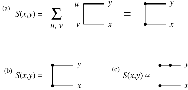
FIG. 4. (a) The diagram for S(x, y) . Thin lines decay with power q_1 and the thick line decays with power q_2 . Unlabelled vertices are summed over. (b) The open triangle diagram for percolation ( q_1 = q_2 = q ). (c) The open square diagram for lattice trees and lattice animals ( q_1 = q, q_2 = 2q - d ).
