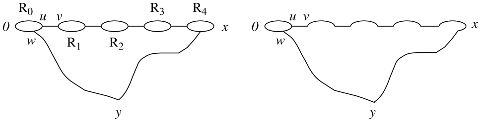
FIG. 7. Configuration for the lattice animal one-loop diagram.
