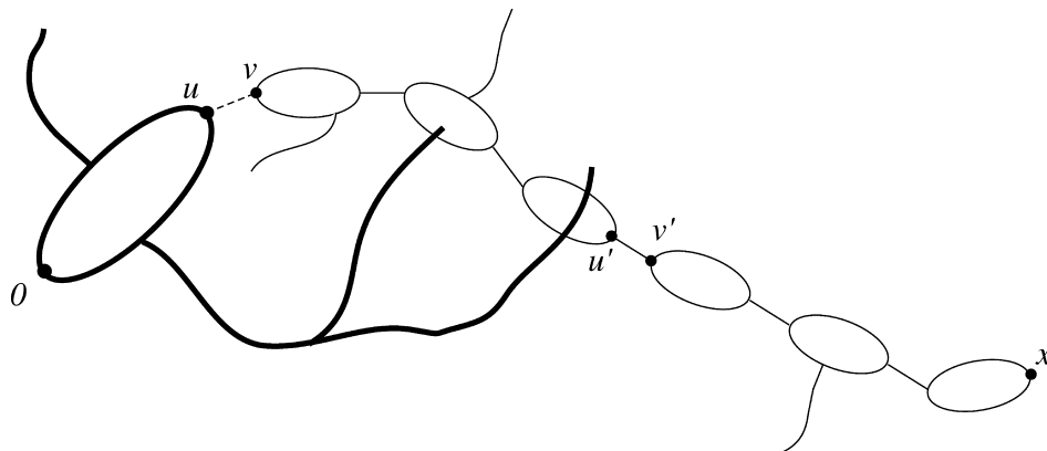
FIG. 2. Schematic representation of the two configurations in a contribution to the nested expectation of (3.24). Bold lines represent occupied bonds in the outer expectation, while thin lines represent occupied bonds in the inner expectation.
